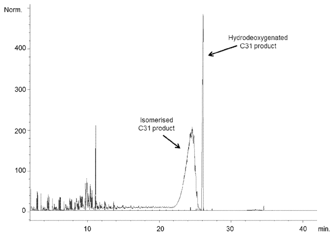
Figure 5 – FIMS analysis of C 31 base oil
