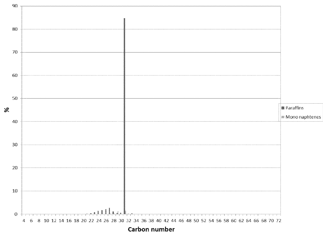
Figure 5 – FIMS analysis of C 31 base oil
