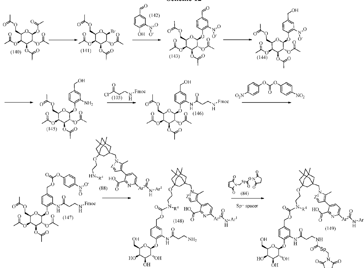
Scheme 12
