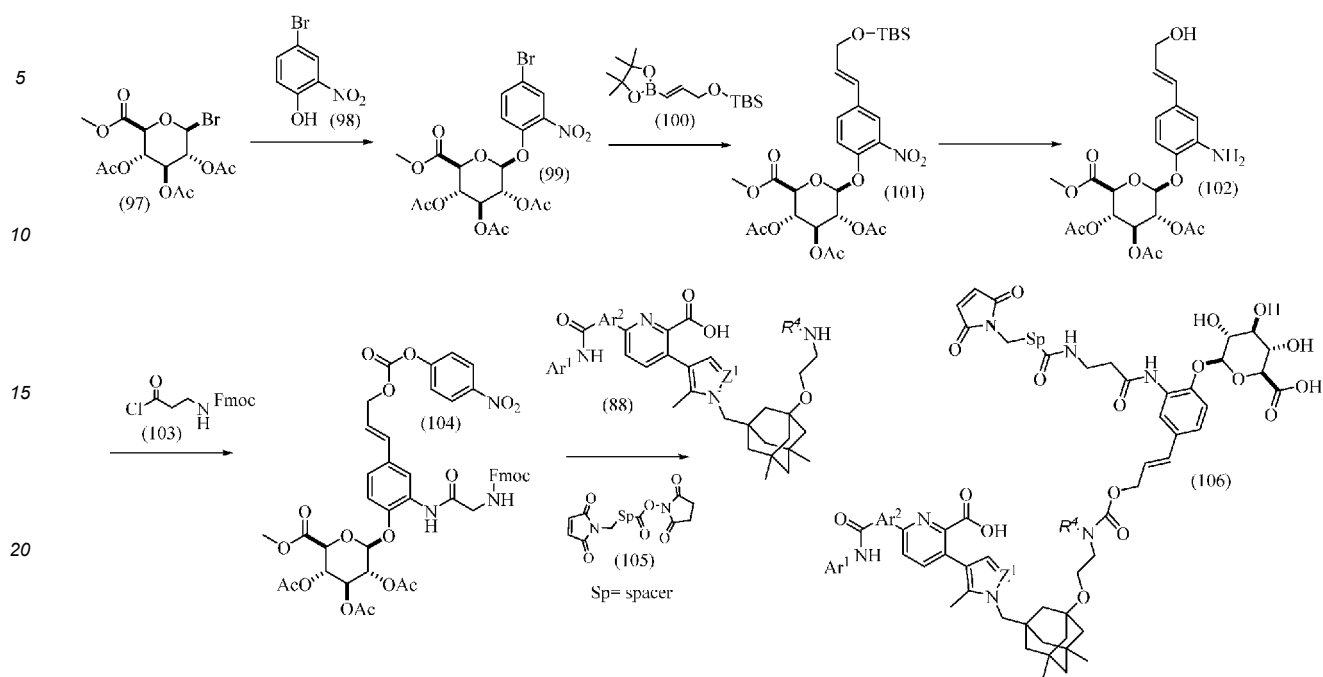
Scheme 7
