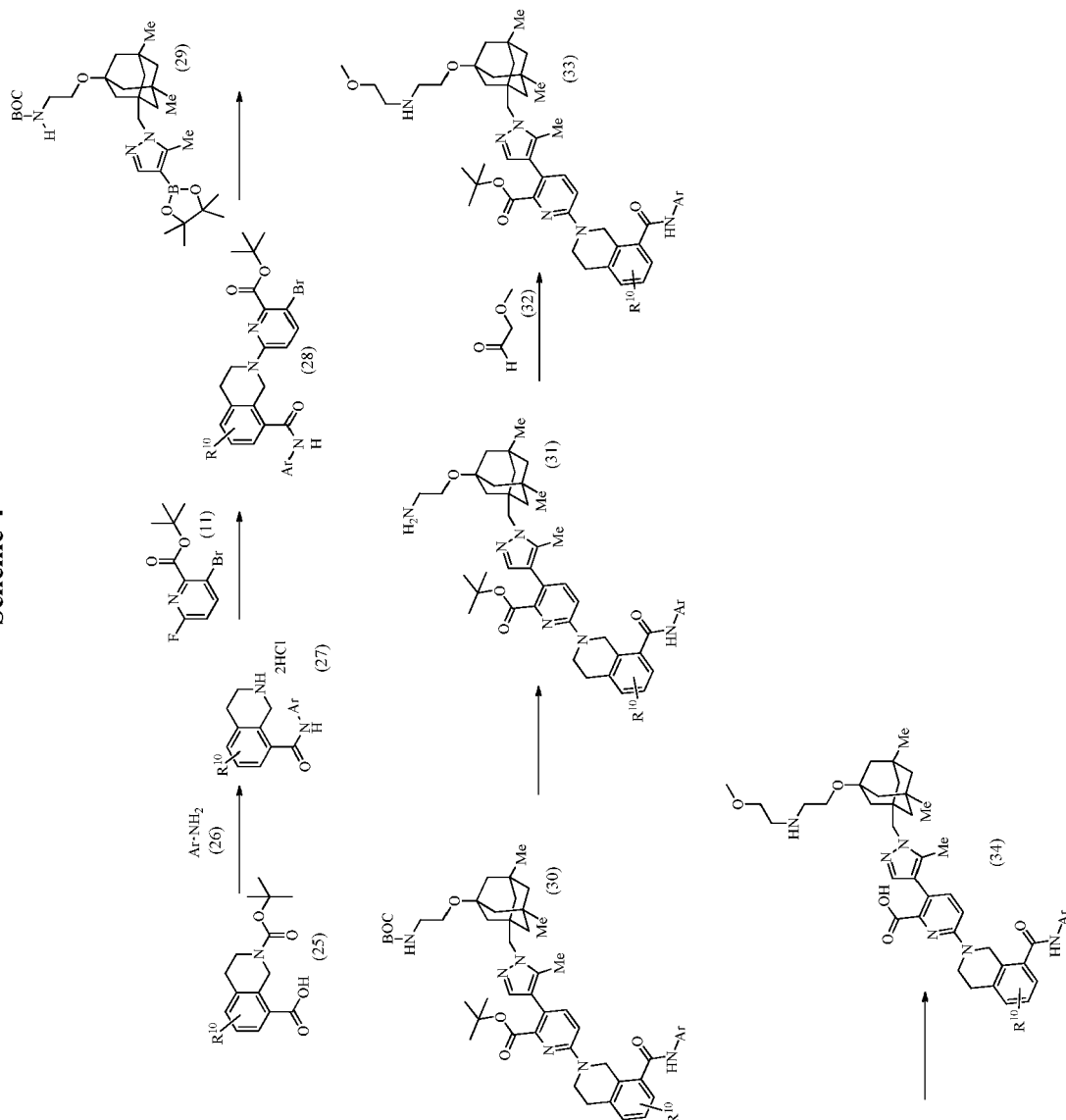
Scheme 4
