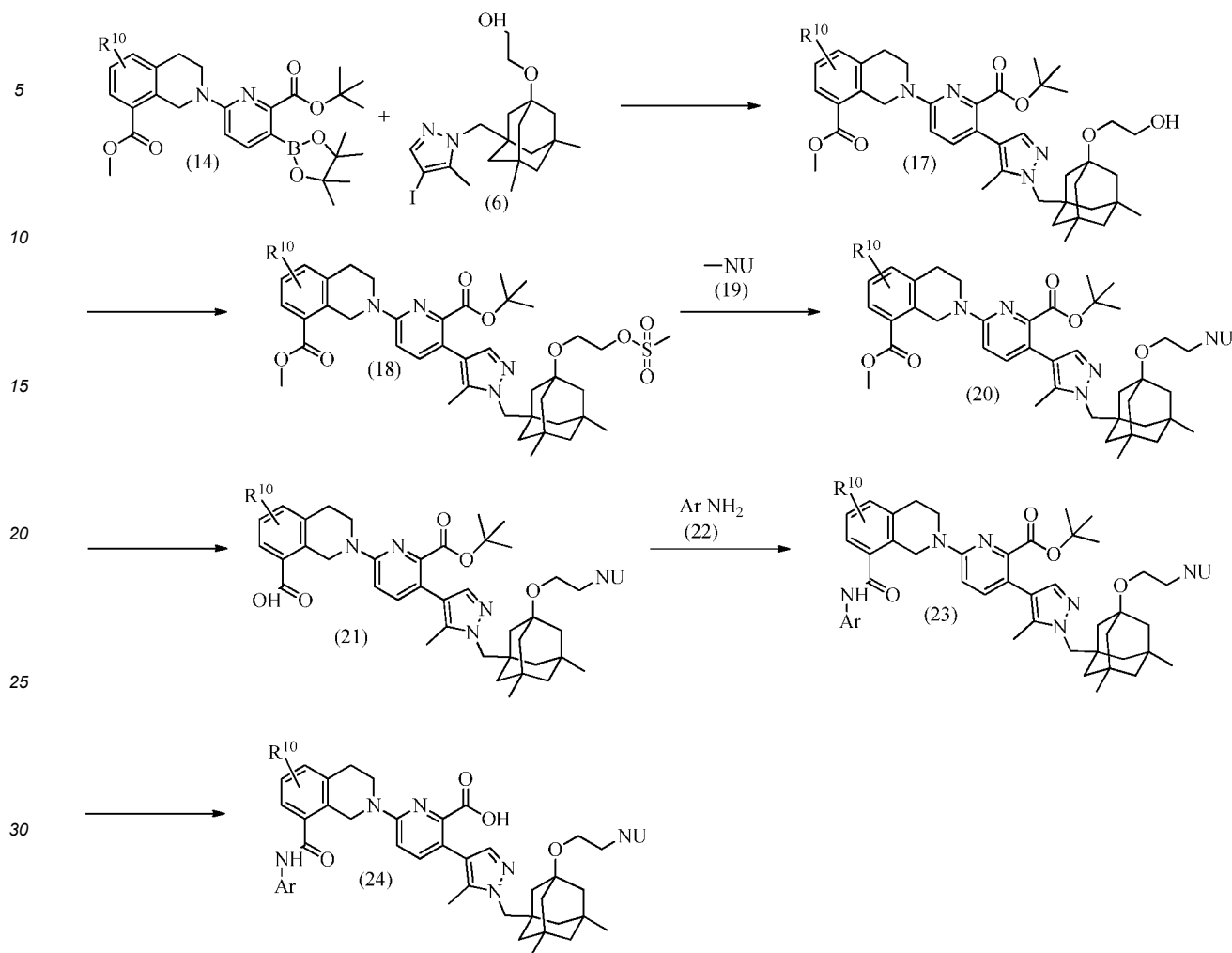
Scheme 3
