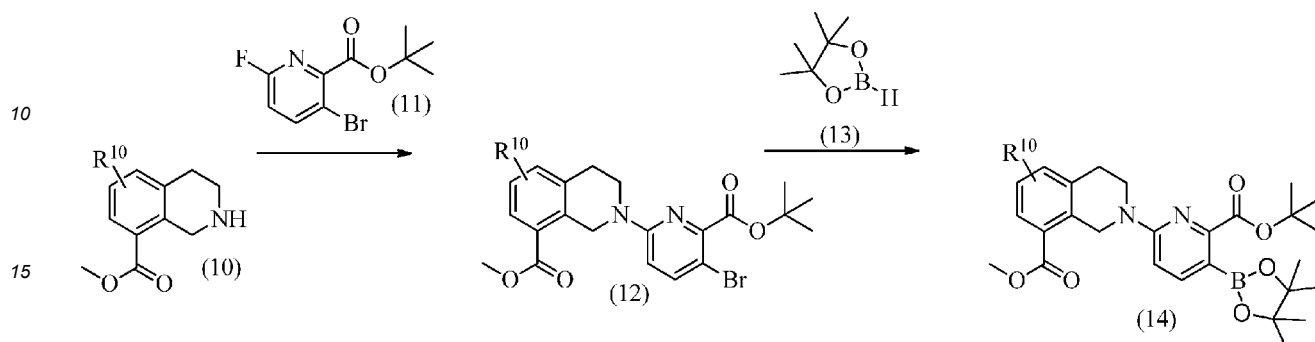
Scheme 2
