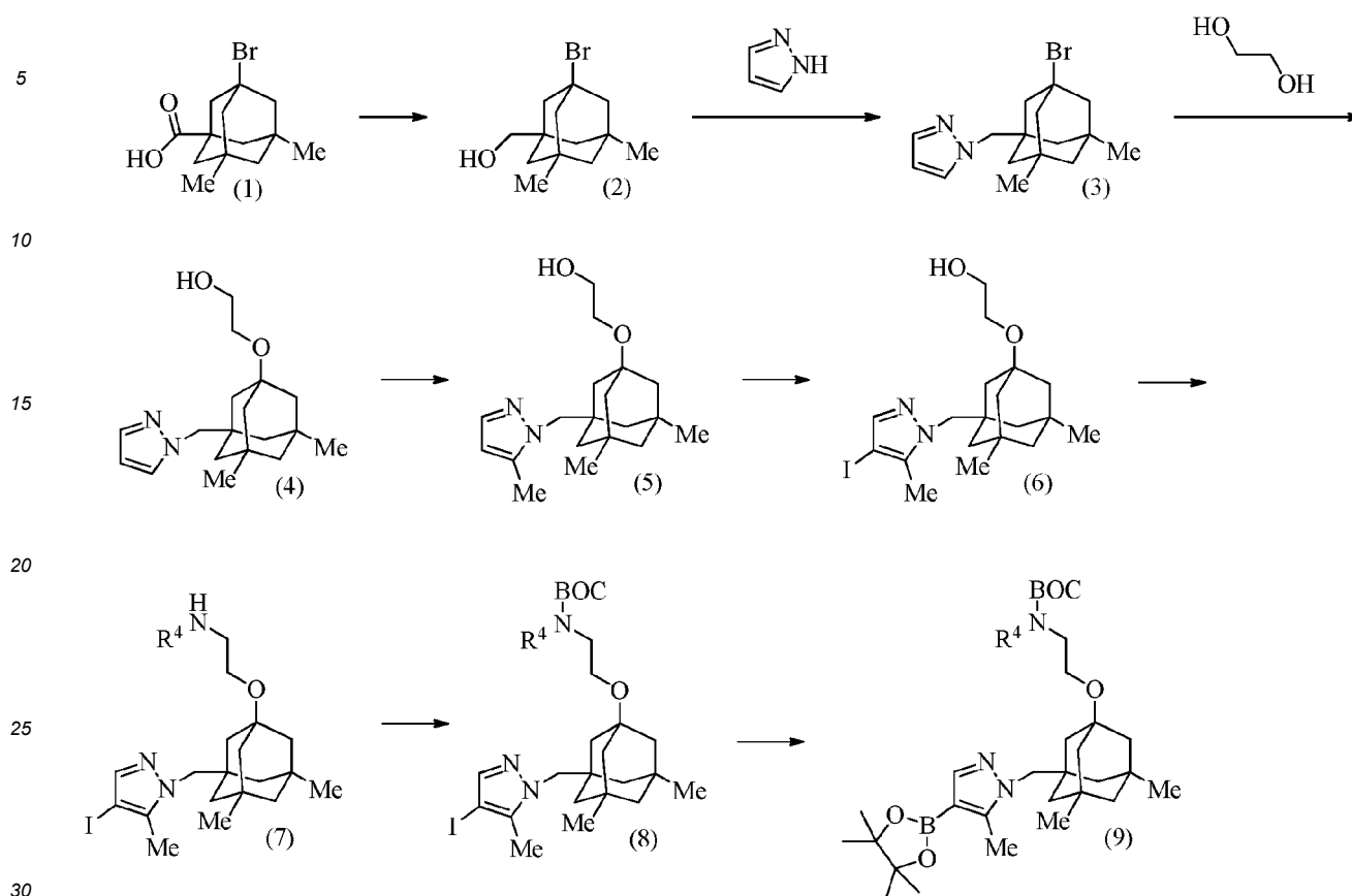
Scheme 1
