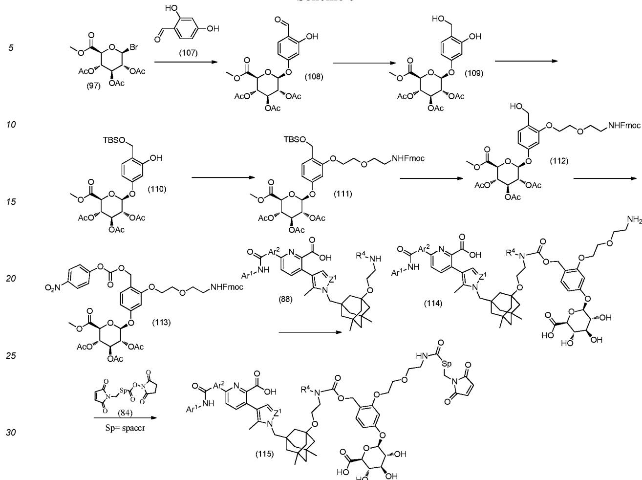
Scheme 8
