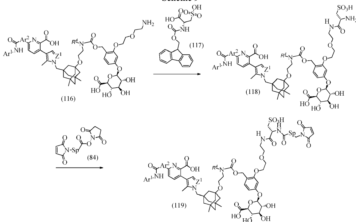
Scheme 9
