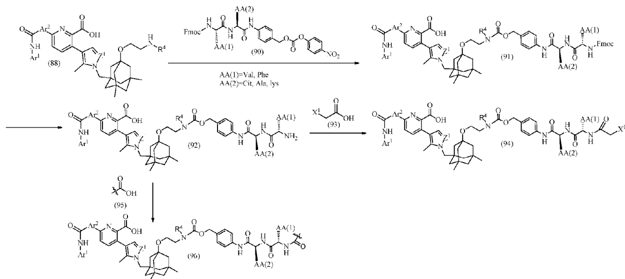
Scheme 6
