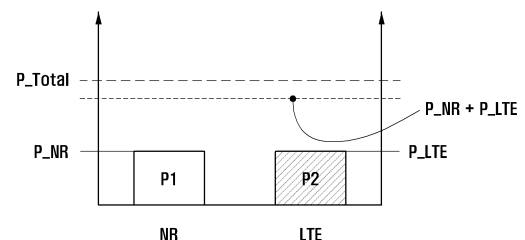
[a] illustration for P_{NR} + P_{LTE} < P_{Total}
