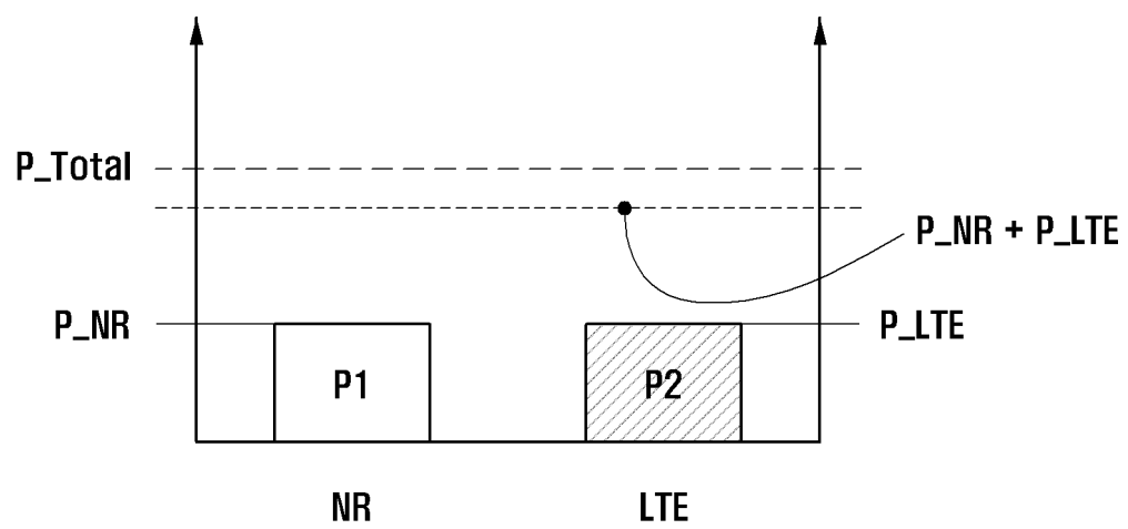
(a) illustration for P_{NR} + P_{LTE} < P_{Total}
