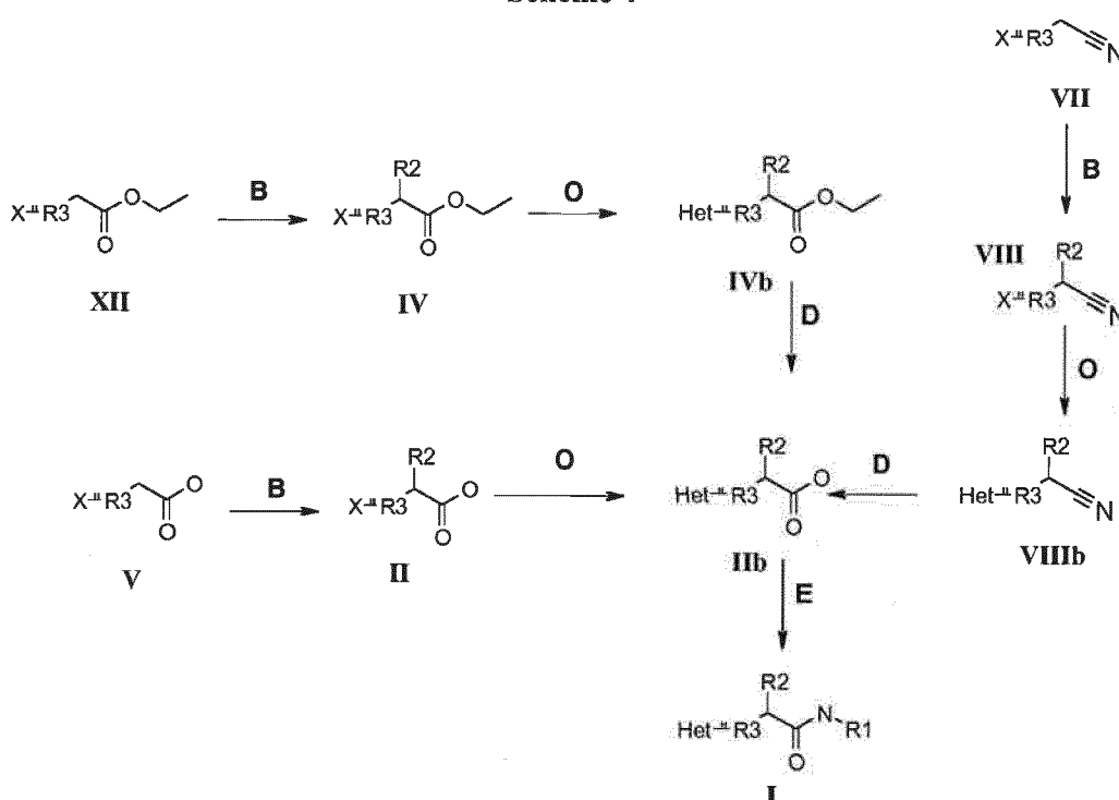
Scheme 4
