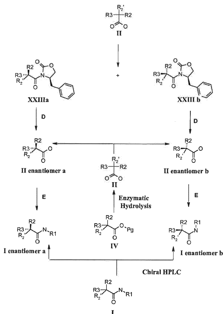
Scheme 5
