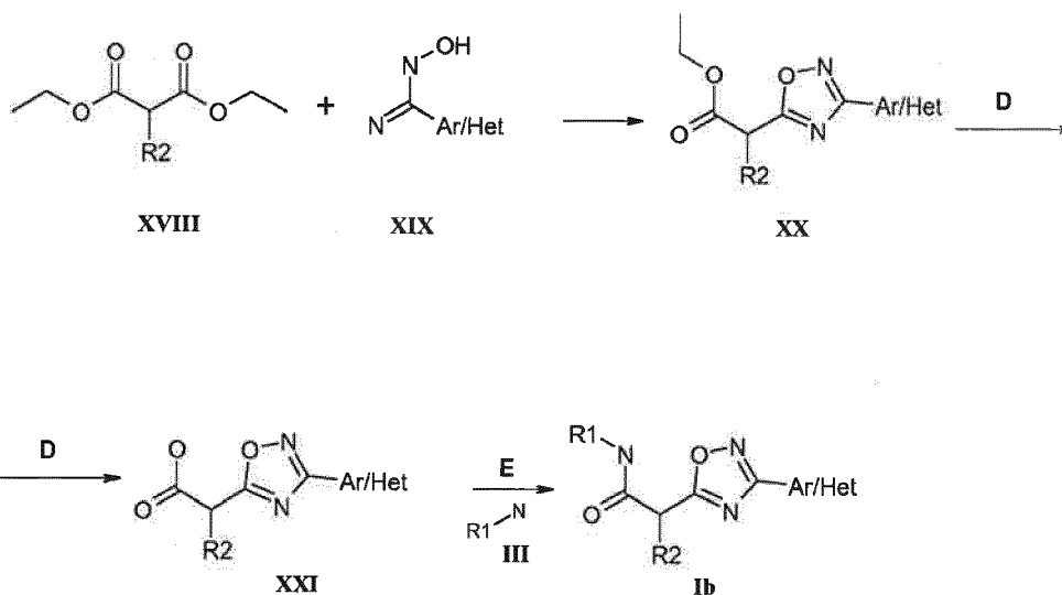
Scheme 2
