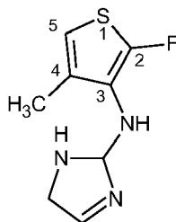
N -(2-fluoro-4-methylthiophen-3-yl)-2,5-dihydro-1 H -imidazol-2-amine
