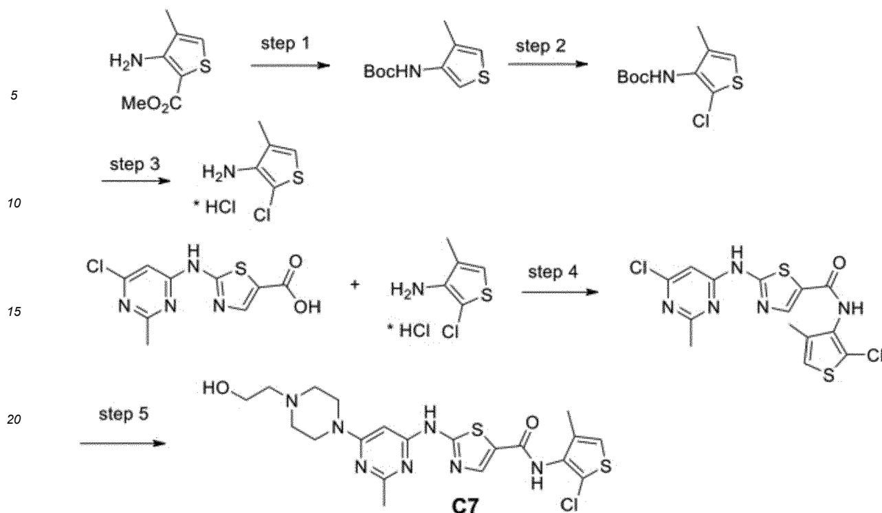
Scheme 2: Synthesis of C7
