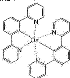
Compound (1 3 2)
