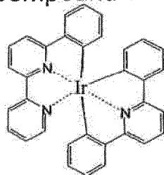
Compound (111)
