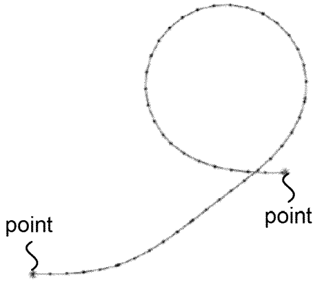
point-to-point
