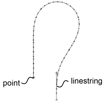
point-to-linestring
