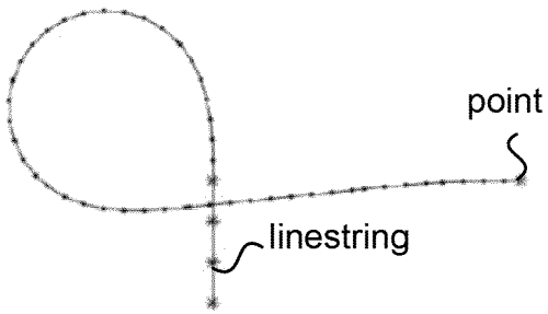
linestring-to-point
