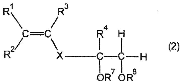
[Chem. 2]
