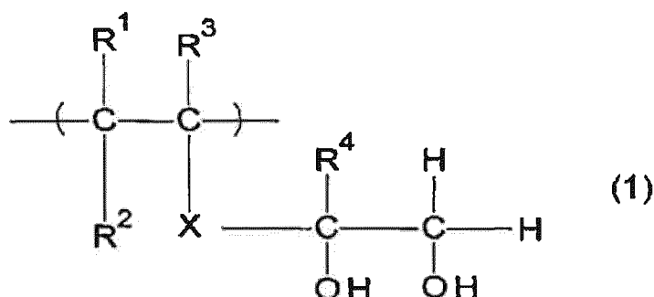
[Chem. 1]
