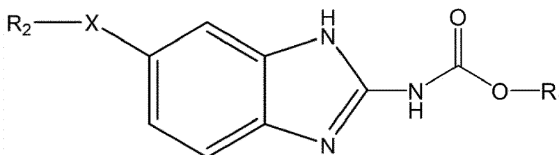
[Chemical Formula 2]
