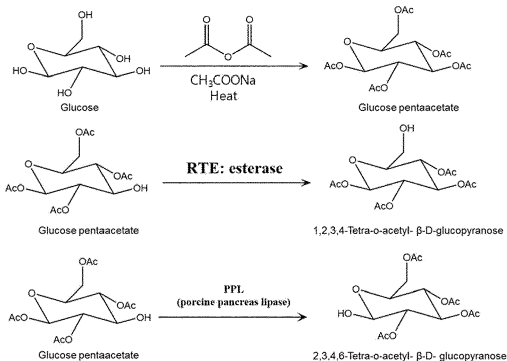
[Reaction Scheme 1]
