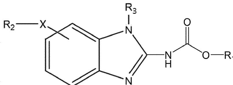
[Chemical Formula 1]
