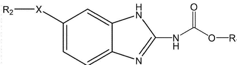
[Chemical Formula 2]
