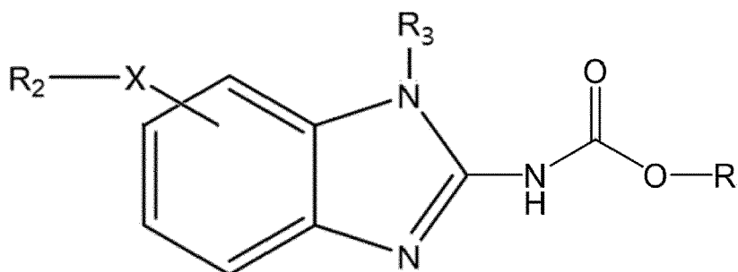
[Chemical Formula 1]
