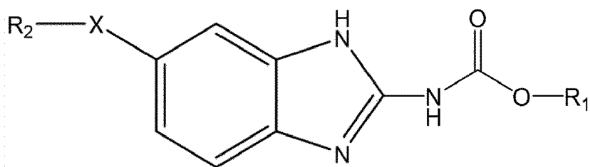
[Chemical Formula 2]
