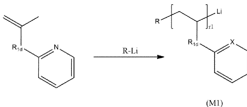
[Reaction 1]
