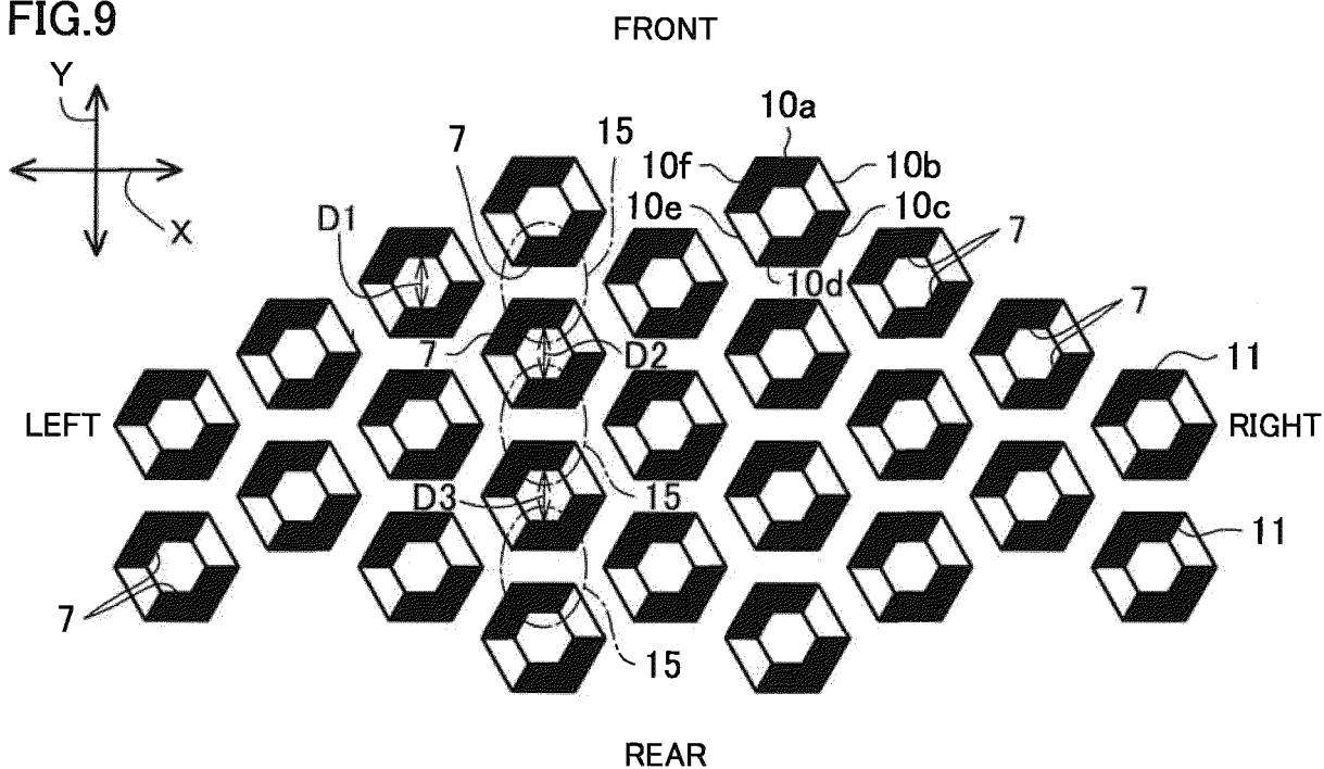
FIRST MODIFICATION OF ARRANGEMENT OF JOINTS
