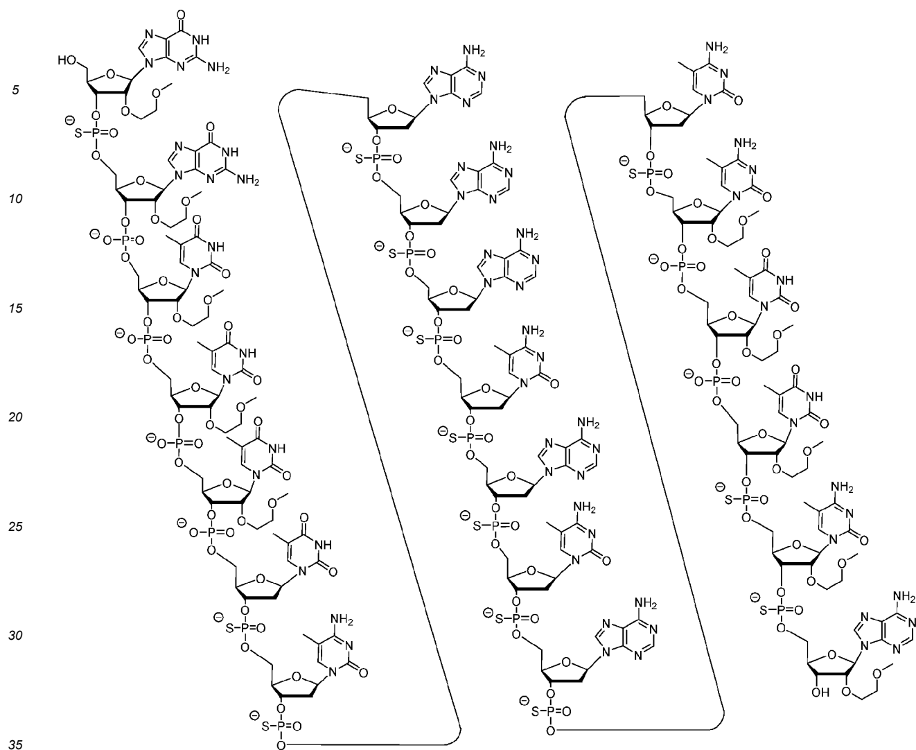
(IIIa)
