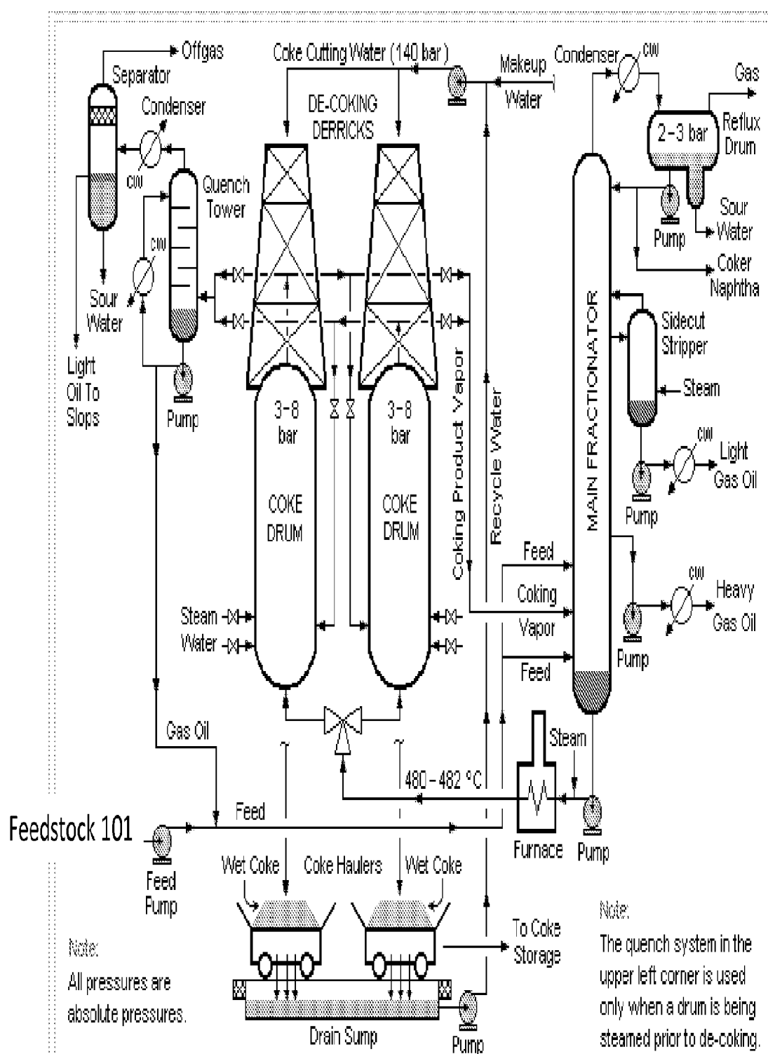
Figure 4 schematic flow diagram of a delayed coking unit
