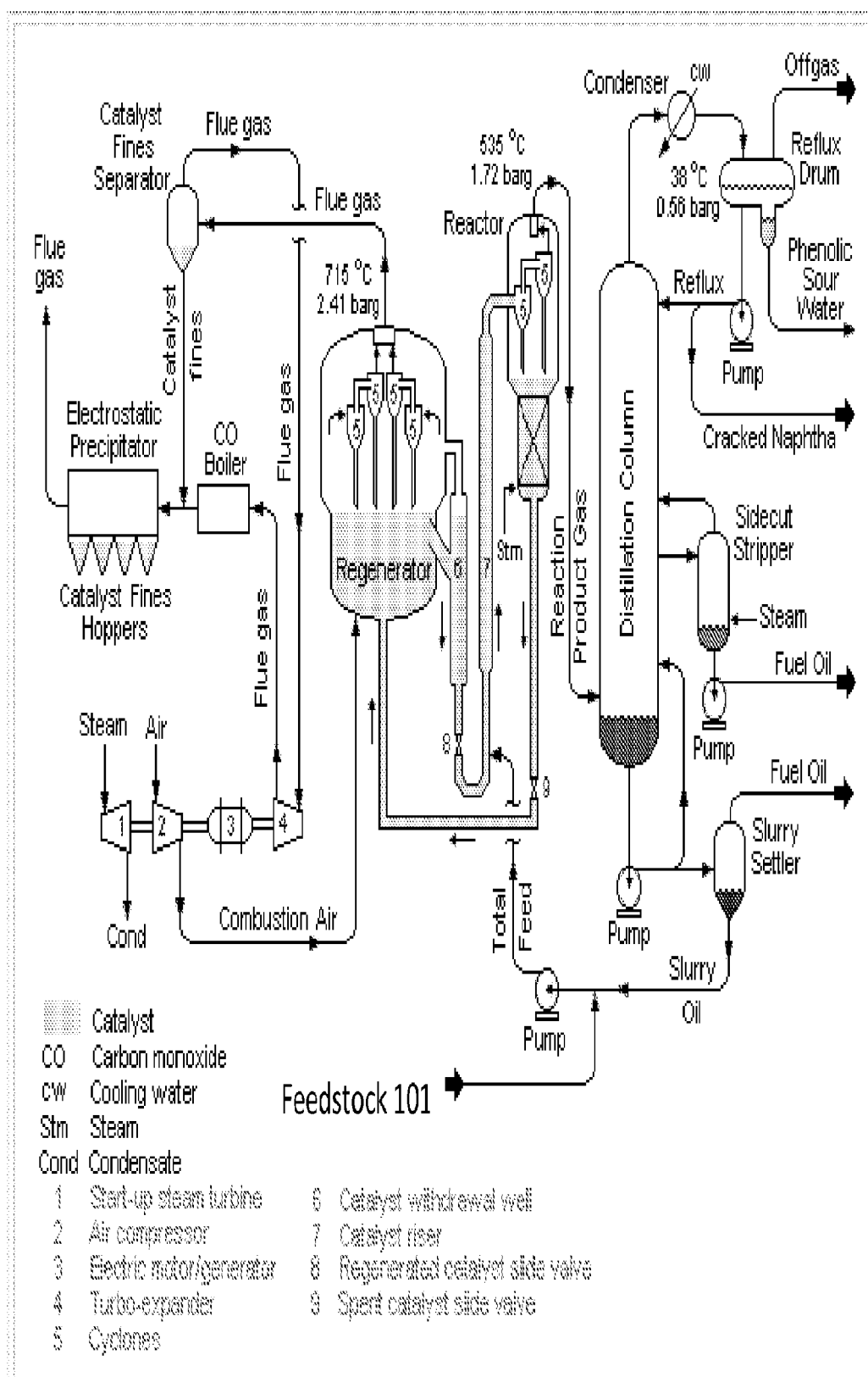
Figure 1 : A schematic flow diagram of a Fluid Catalytic Cracking unit as used in petroleum refineries
