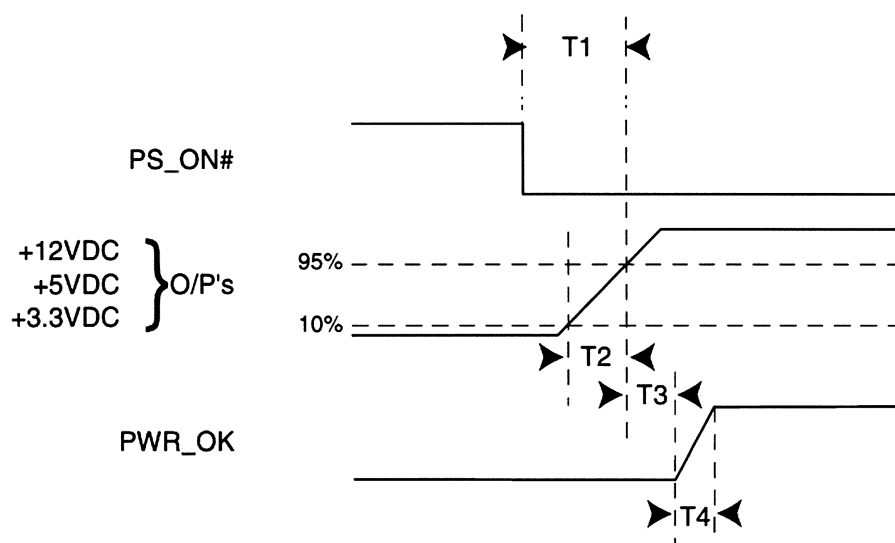
Figure 2 (Prior Art)
