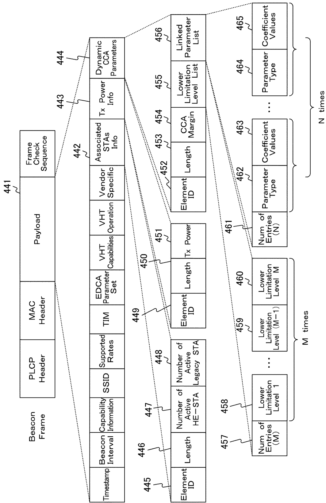
FIG. 17 EXAMPLE OF FORMAT OF BEACON
