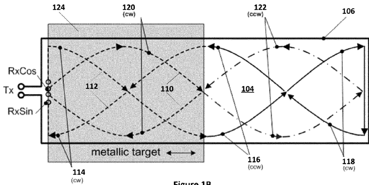
Figure 1B (Prior Art)
