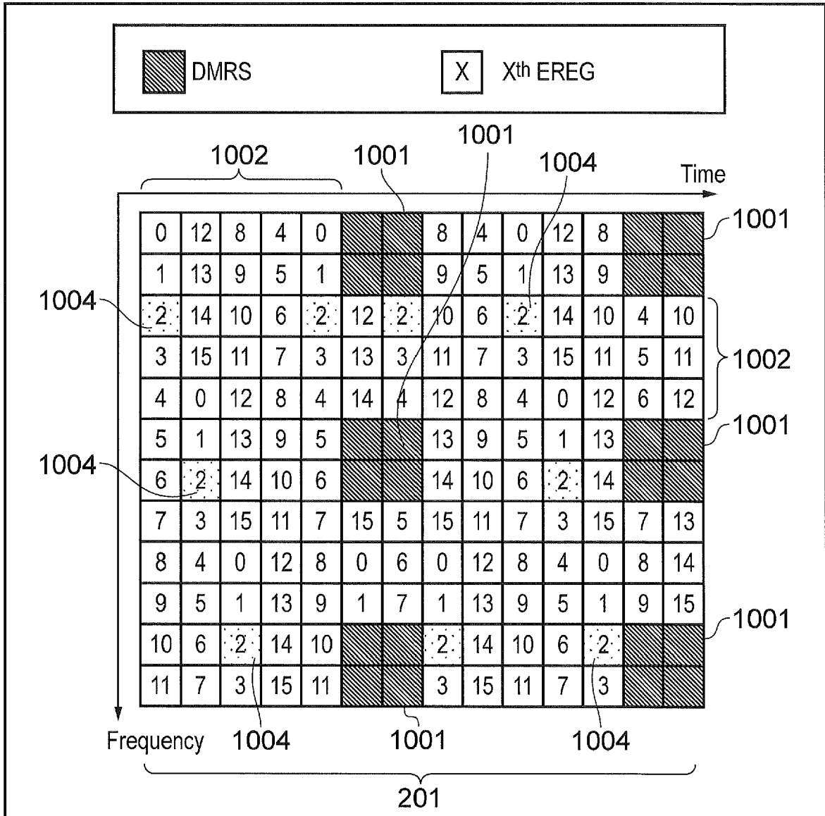
Mapping of eREGs to Res
