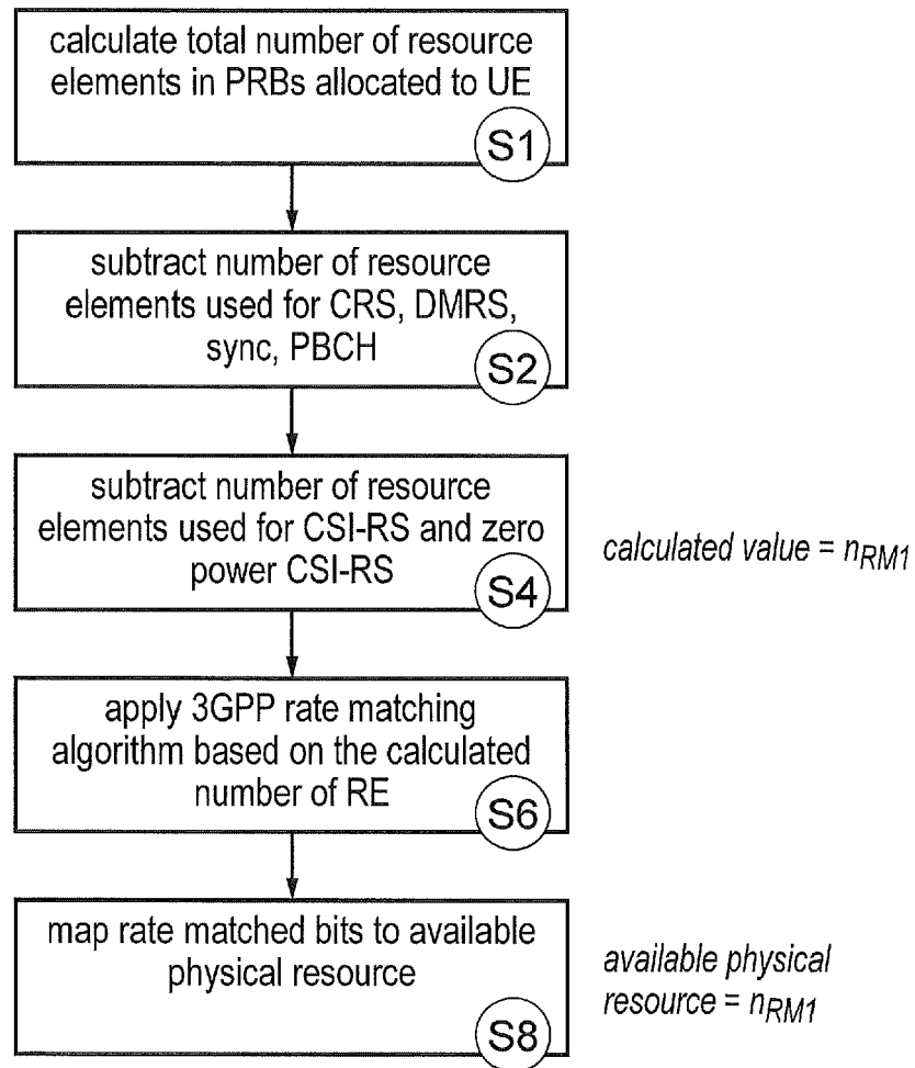
Flow chart of operation of rate matching when applied to subframes containing CSI-RS
