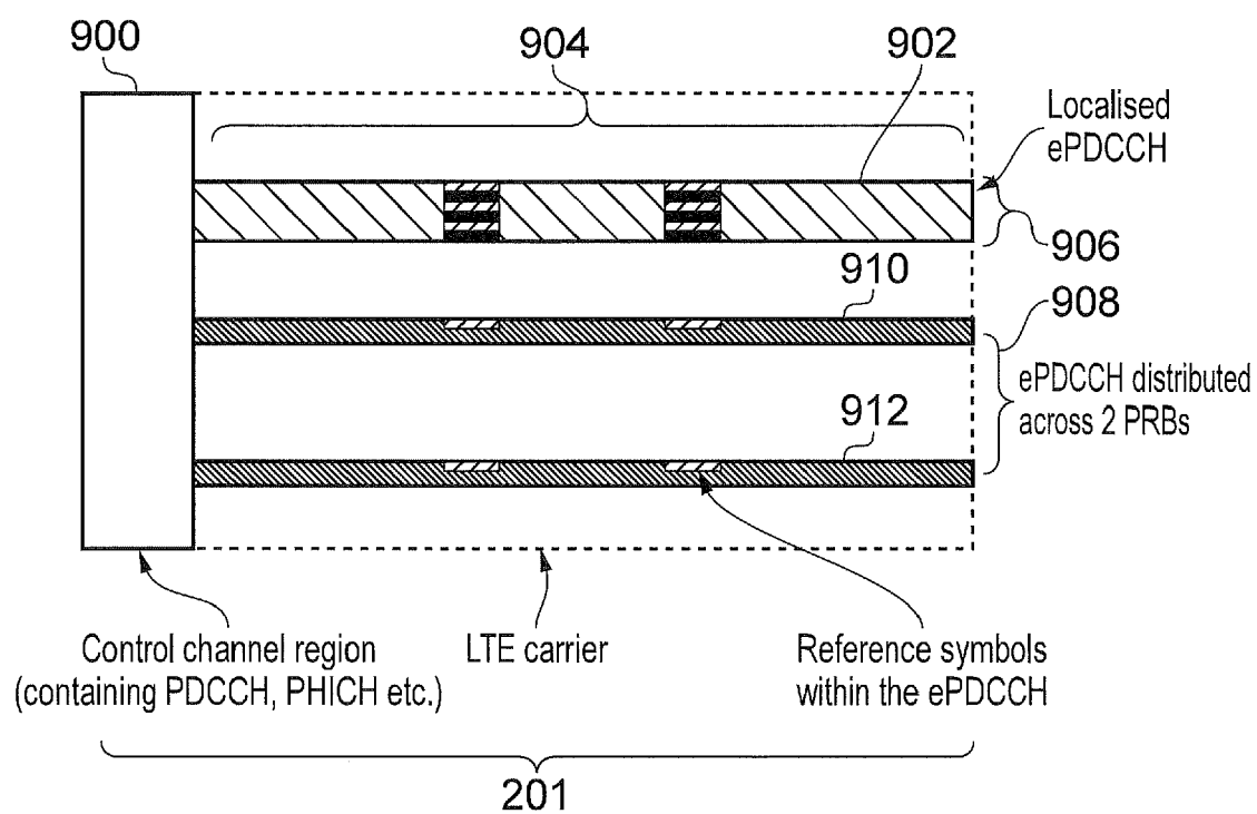
Localised and distributed forms of ePDCCH
