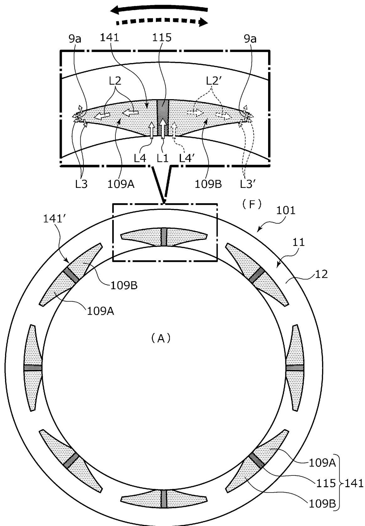
Fig. 6 ROTATIONAL DIRECTION OF ROTATING SEAL RING
