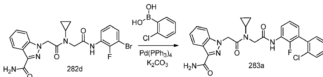
Scheme 283
