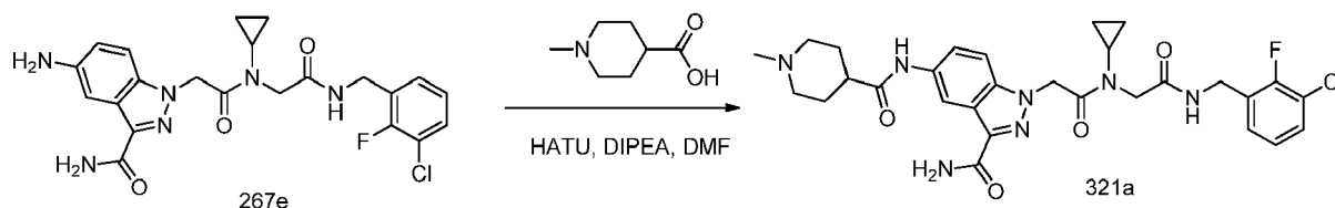
Scheme 321
