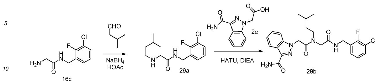
Scheme 29
