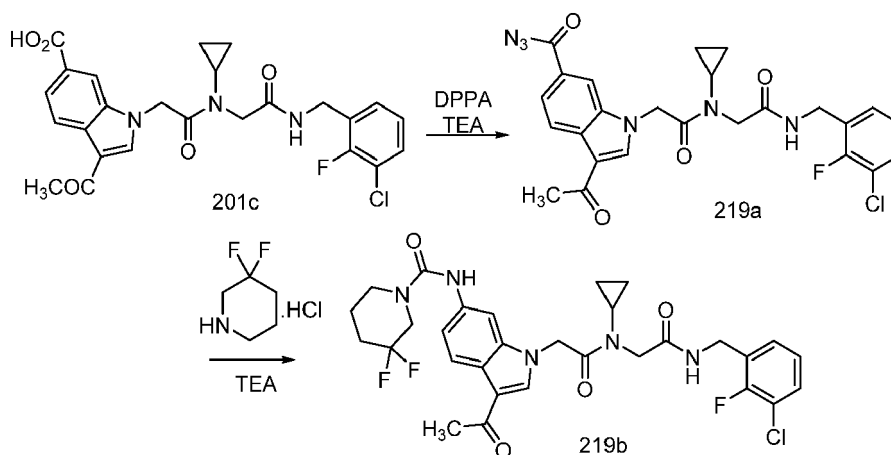
Scheme 219
