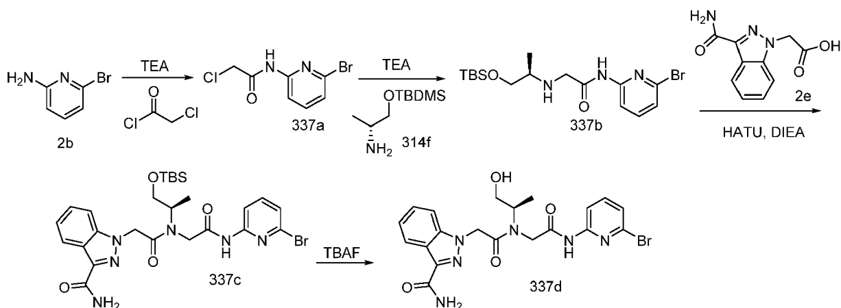
Scheme 337
