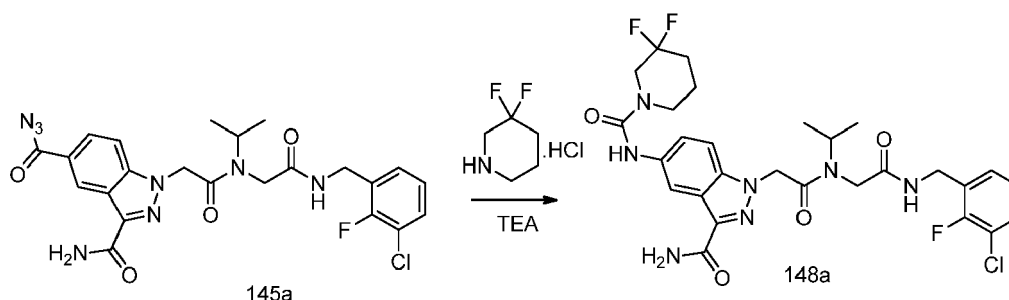
Scheme 148
