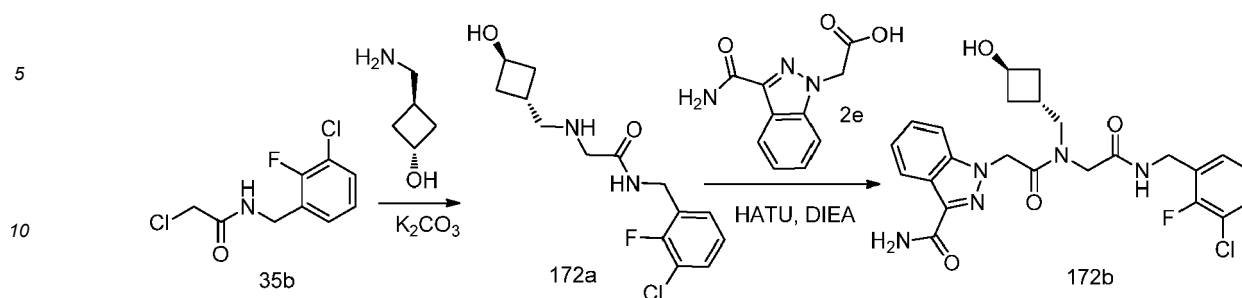
Scheme 172
