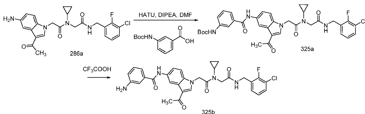
Scheme 325
