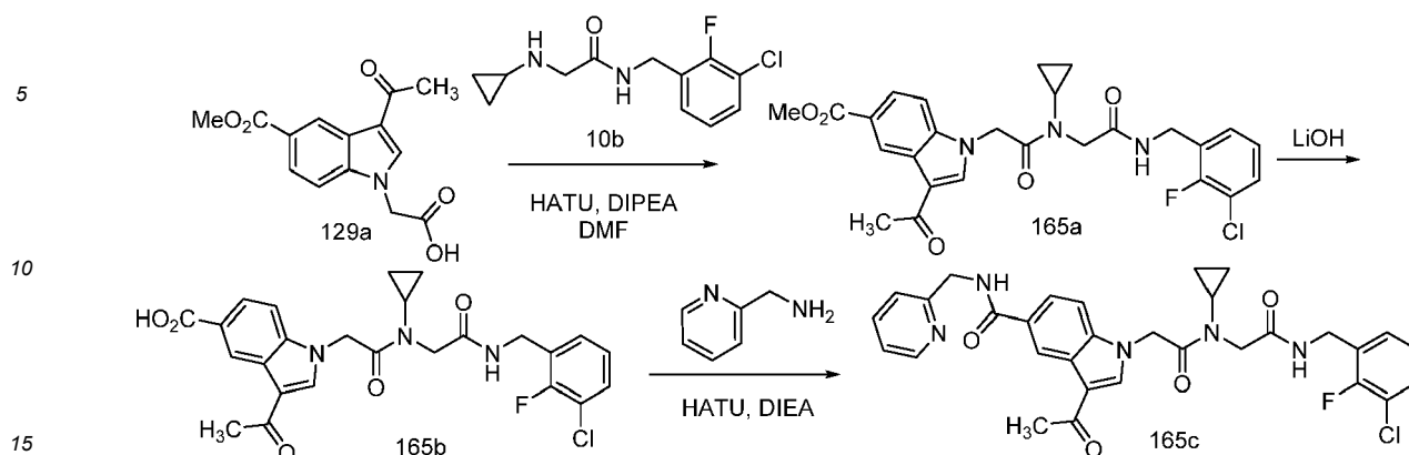
Scheme 165
