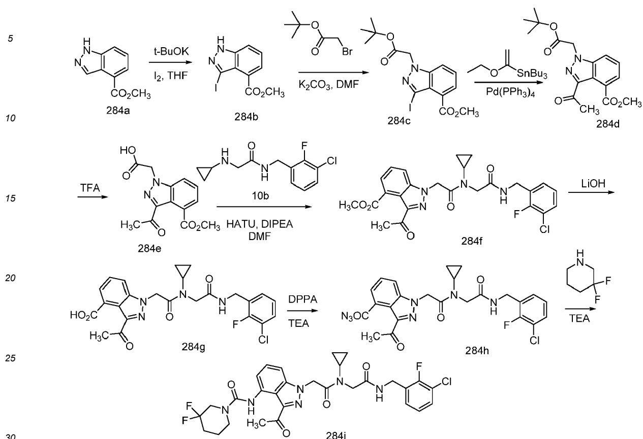
Scheme 284
