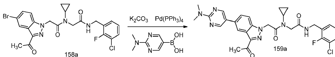
Scheme 159
