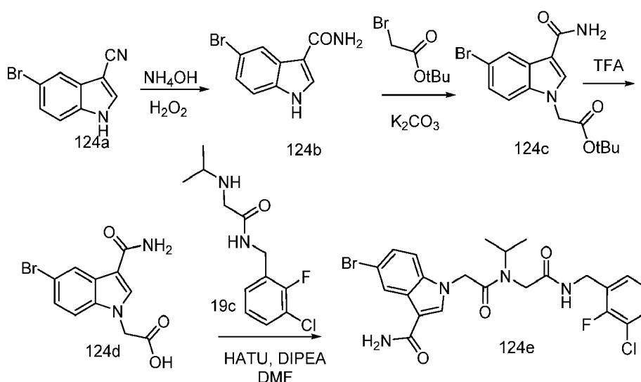
Scheme 124
