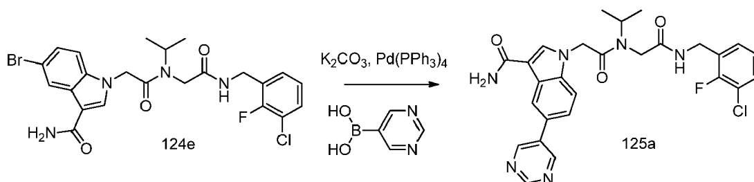
Scheme 125
