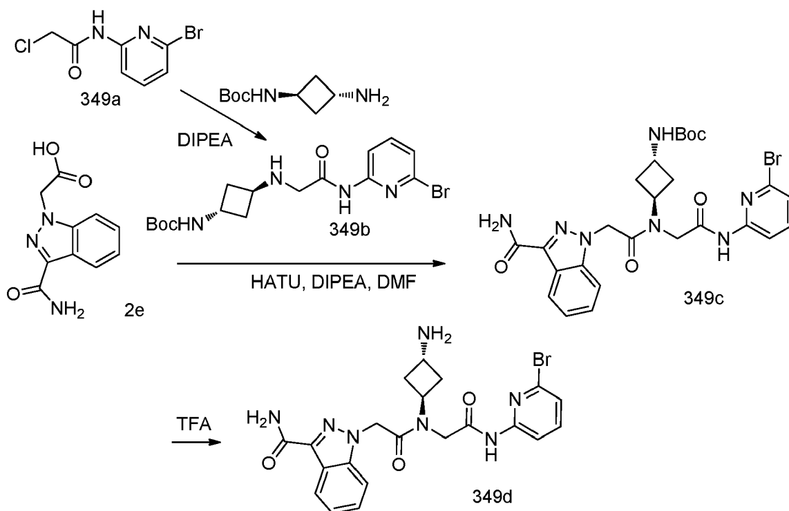
Scheme-349
