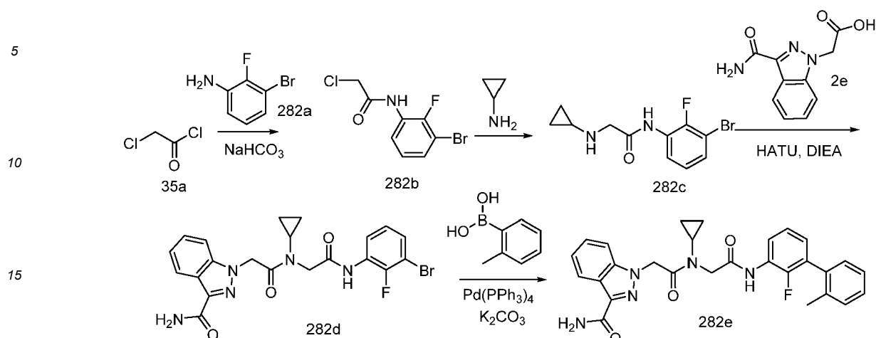
Scheme 282
