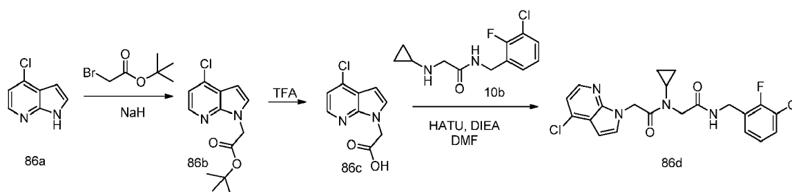
Scheme 86
