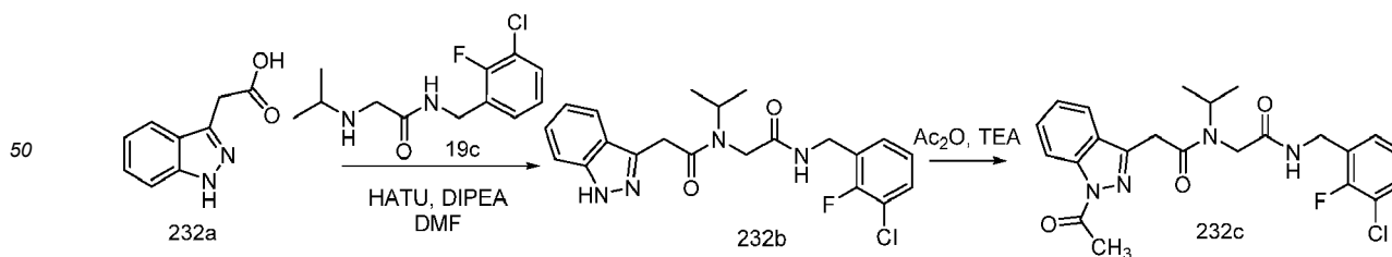
Scheme 232
