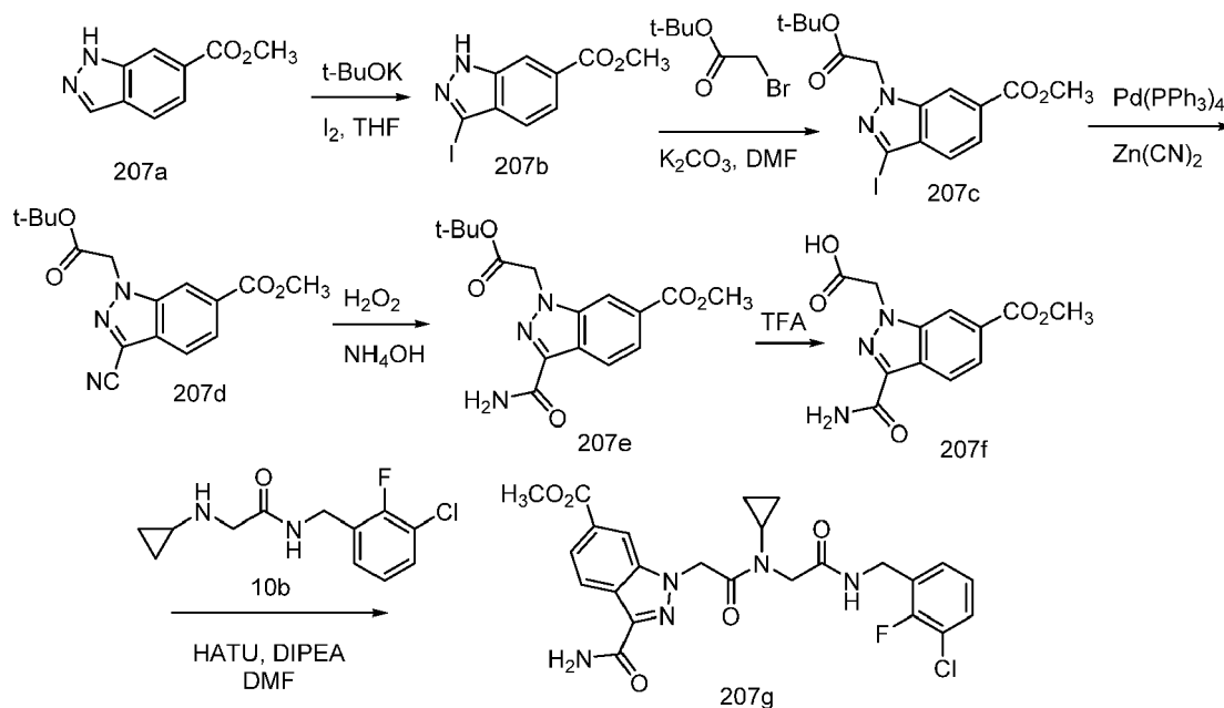
Scheme 207
