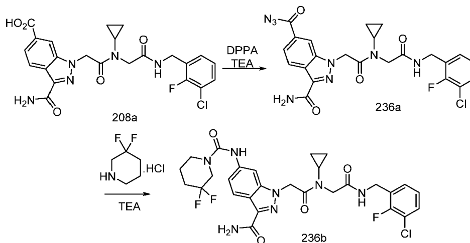
Scheme 236
