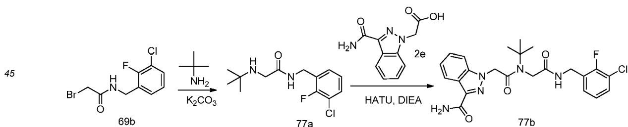
Scheme 77
