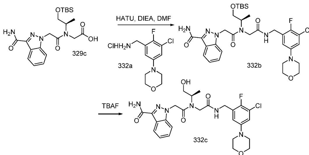
Scheme 332
