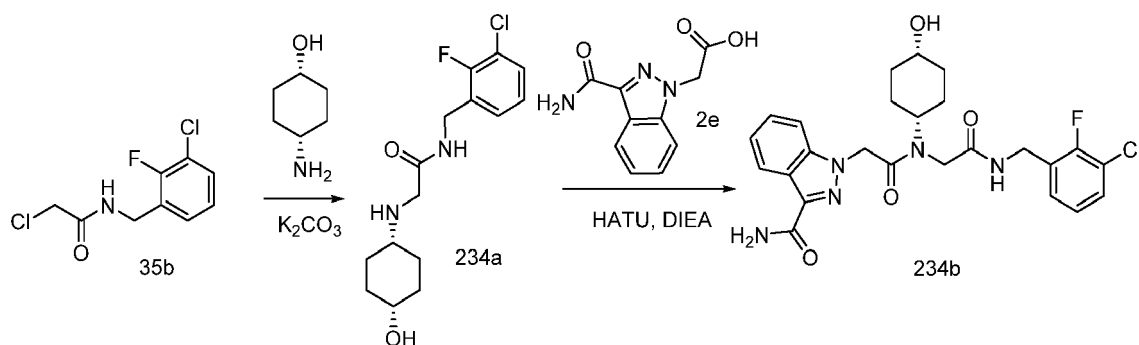
Scheme 234
