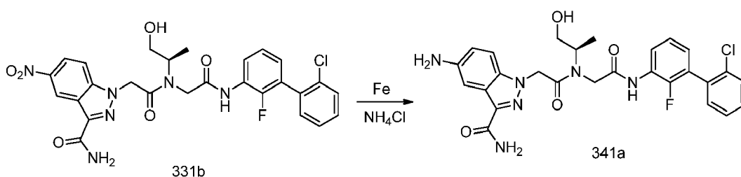
Scheme 341
