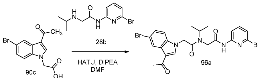
Scheme 96
