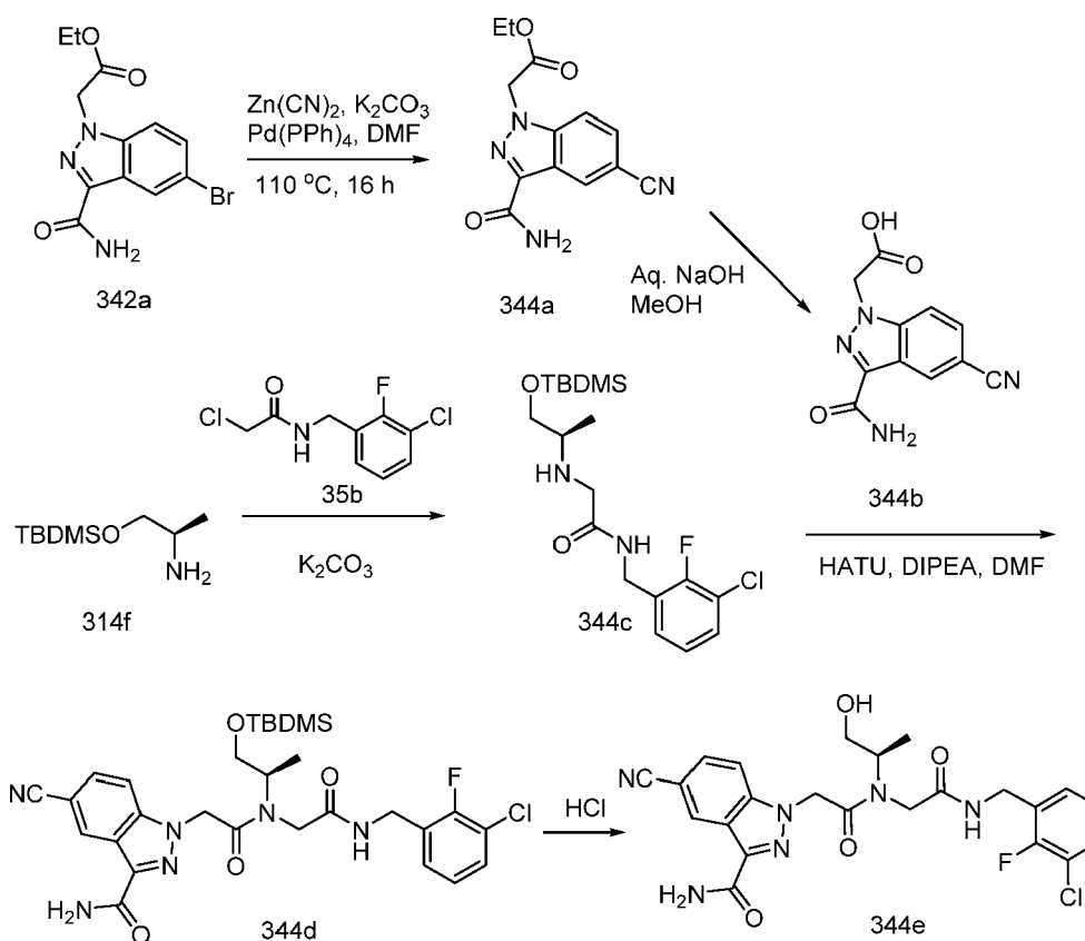
Scheme 344
