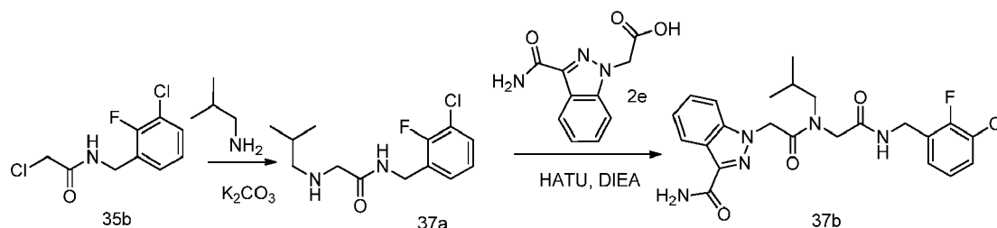
Scheme 37
