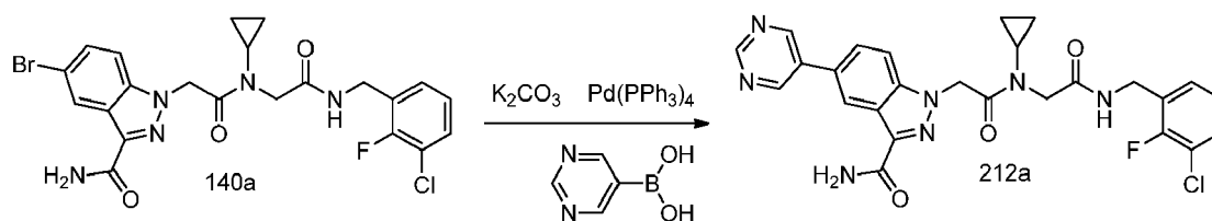
Scheme 212
