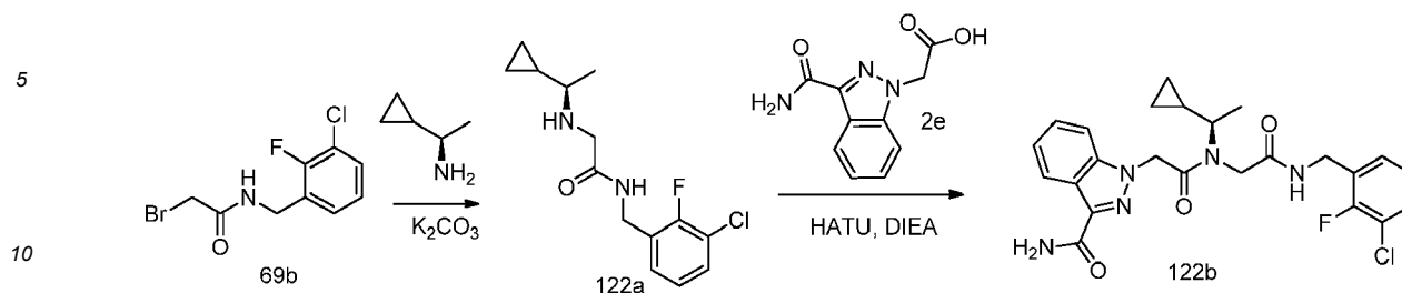
Scheme 122
