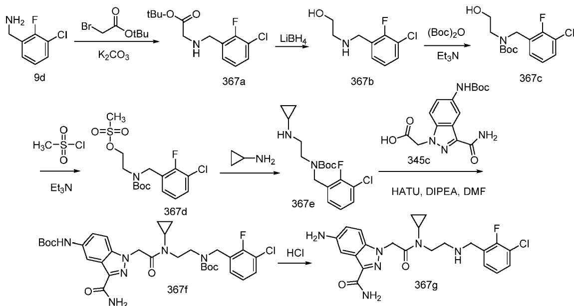
Scheme 367
