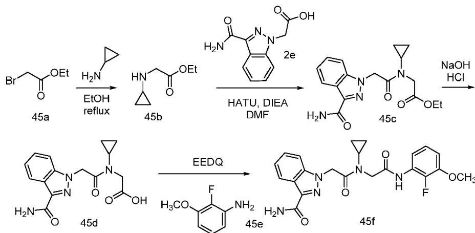
Scheme 45
