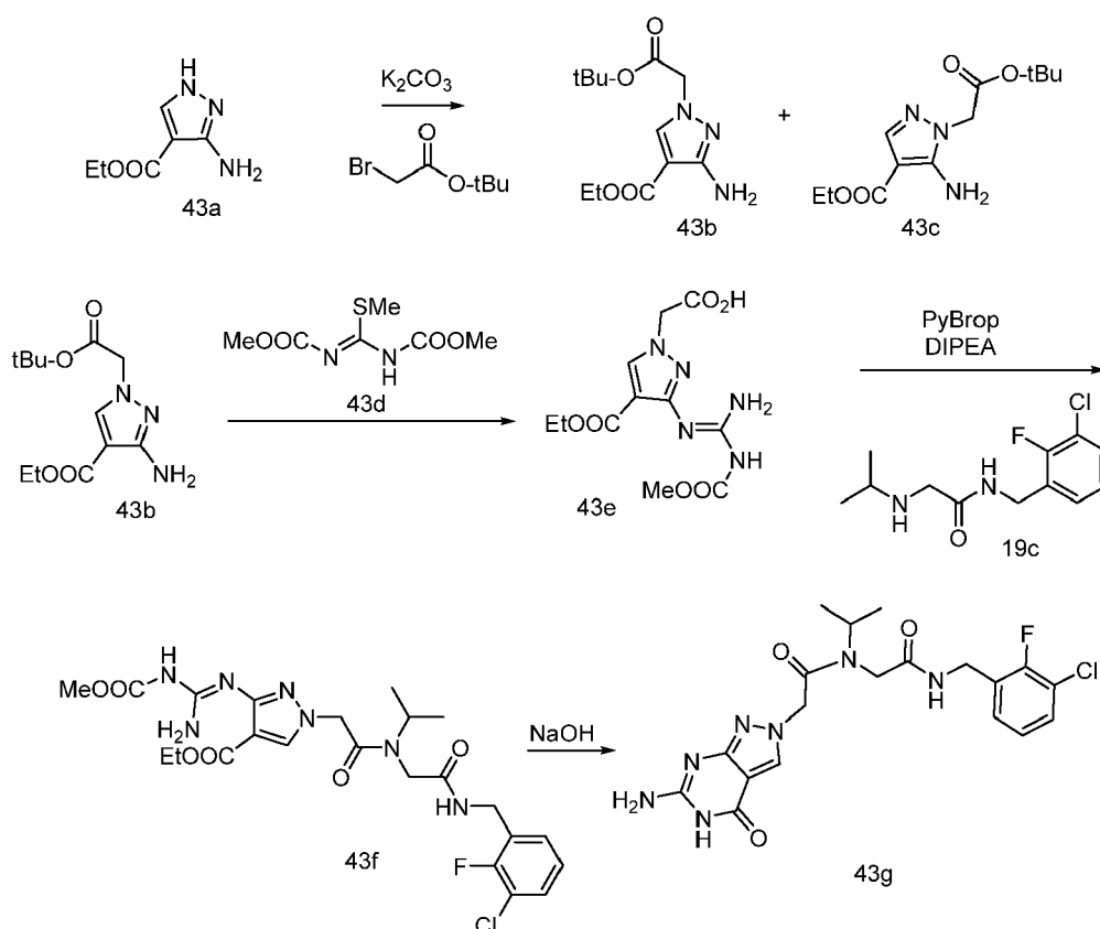
Scheme 43
