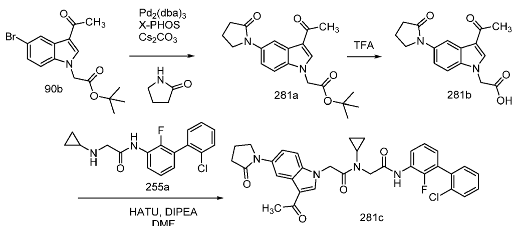
Scheme 281
