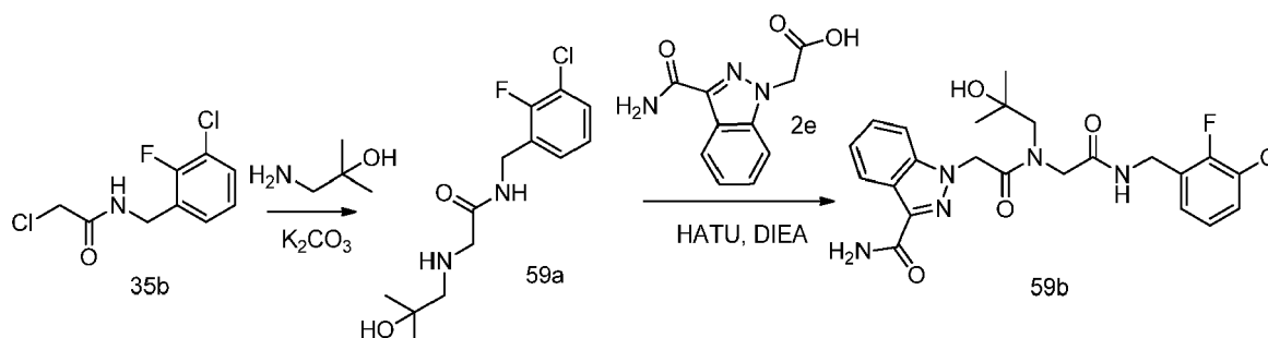
Scheme 59
