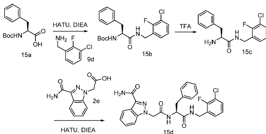
Scheme 15
