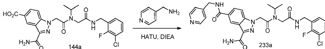
Scheme 233
