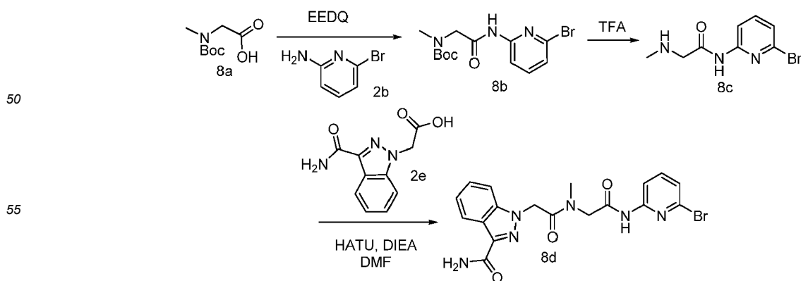
Scheme 8
