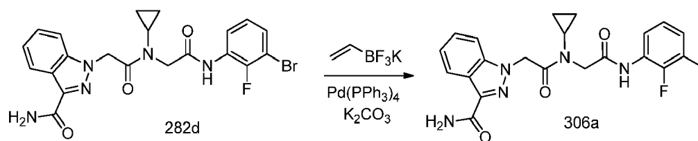
Scheme 306
