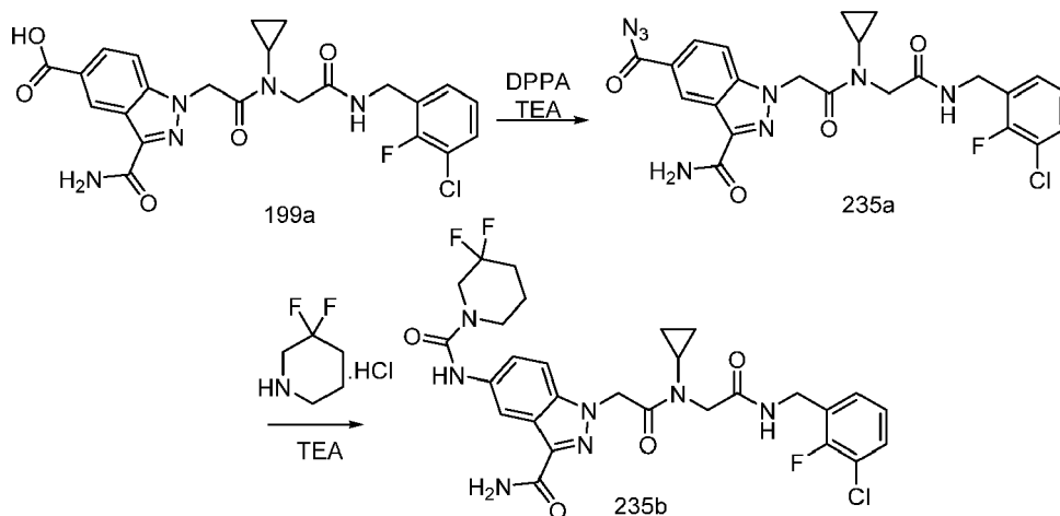
Scheme 235
