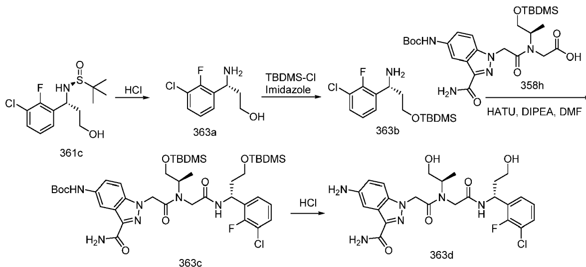
Scheme 363
