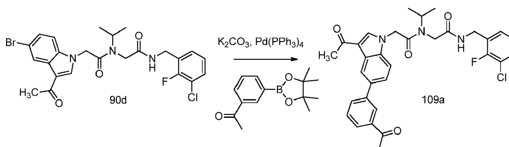
Scheme 109
