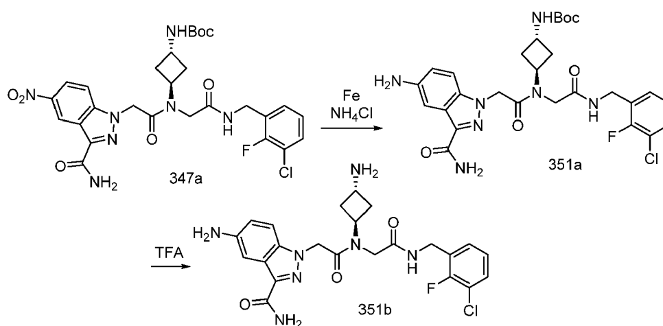
Scheme 351
