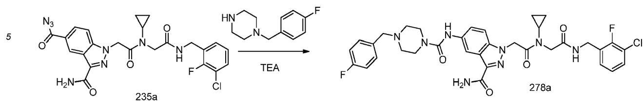
Scheme 278
