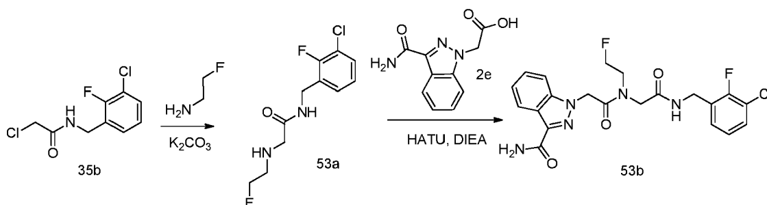
Scheme 53
