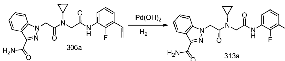
Scheme 313
