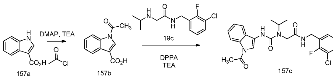
Scheme 157
