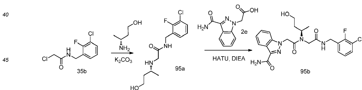
Scheme 95
