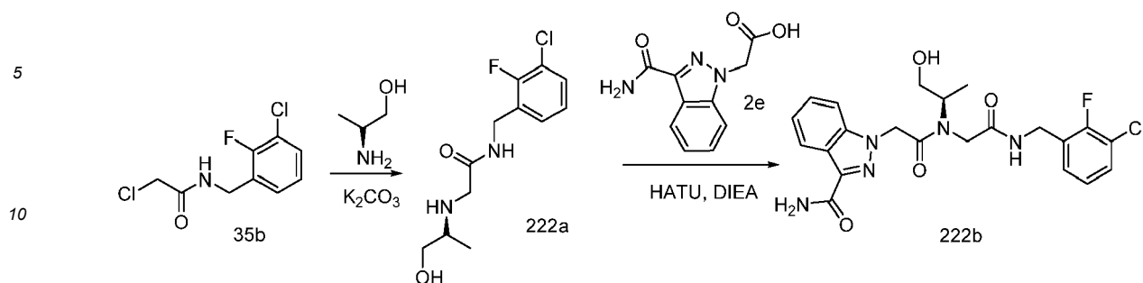
Scheme 222
