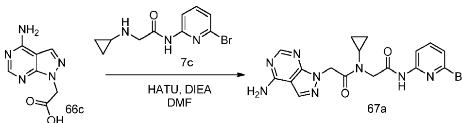
Scheme 67
