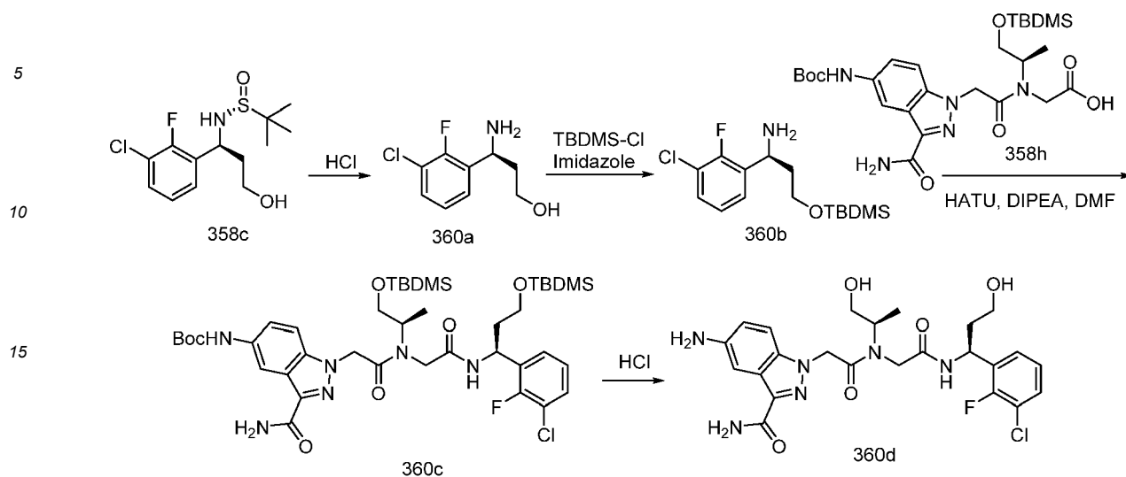
Scheme 360
