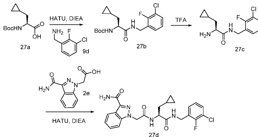
Scheme 27
