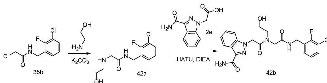
Scheme 42
