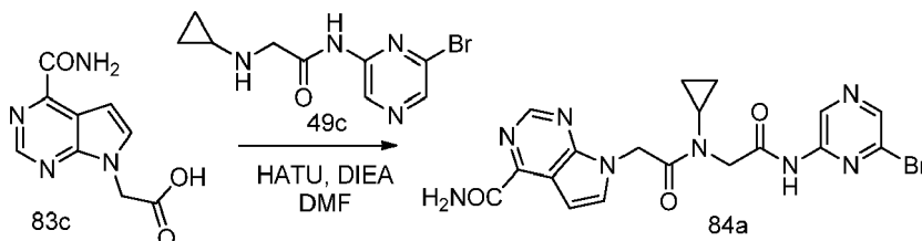
Scheme 84
