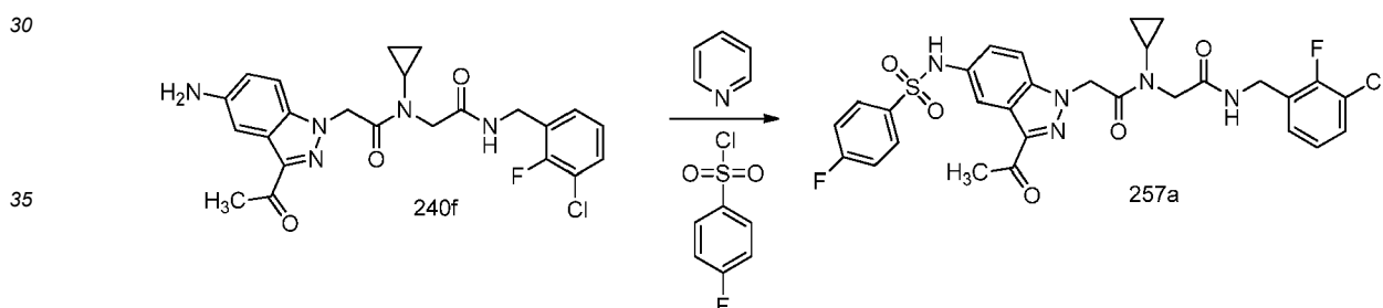
Scheme 257
