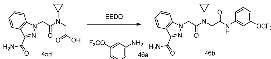
Scheme 46
