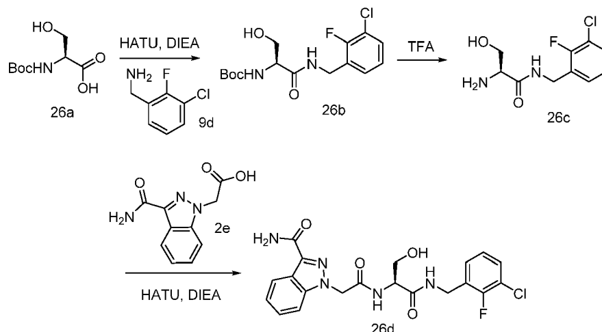
Scheme 26
