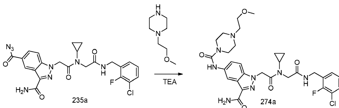
Scheme 274
