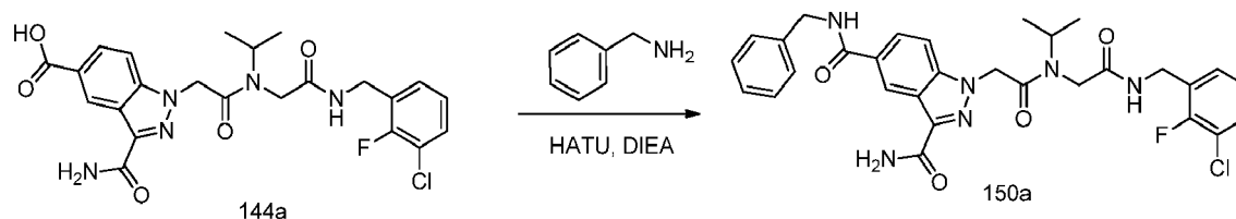
Scheme 150
