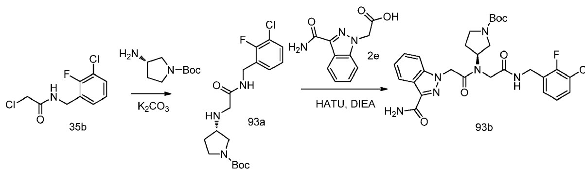
Scheme 93
