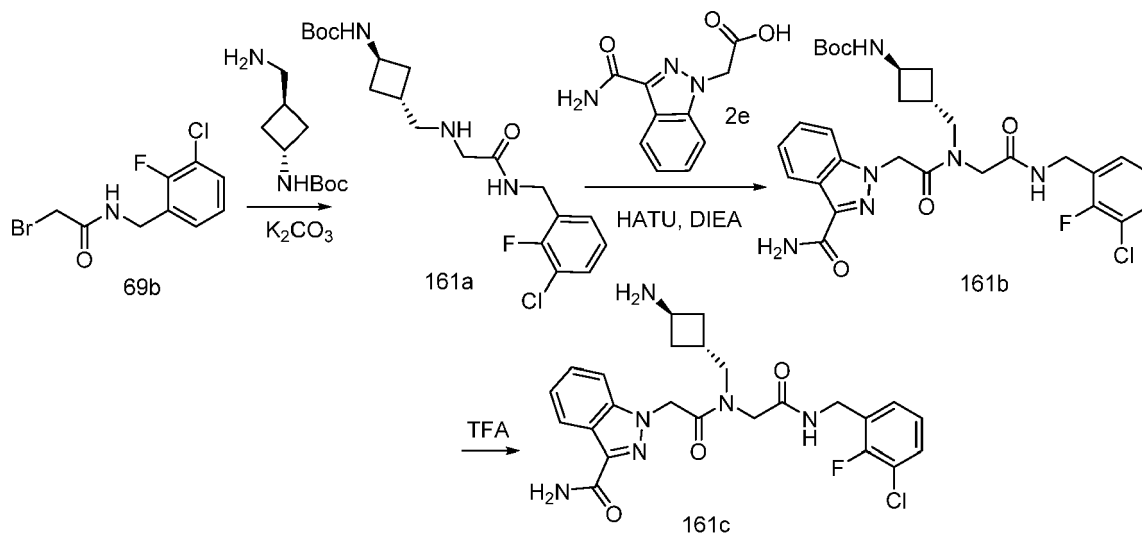
Scheme 161
