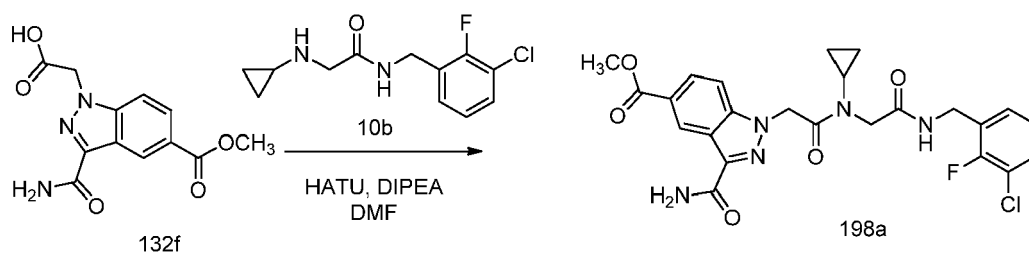
Scheme 198
