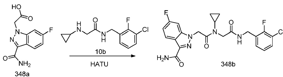
Scheme 348
