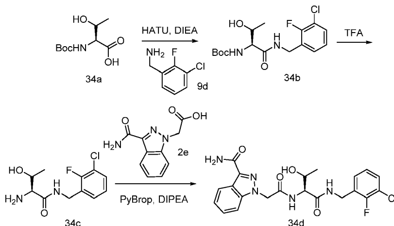
Scheme 34
