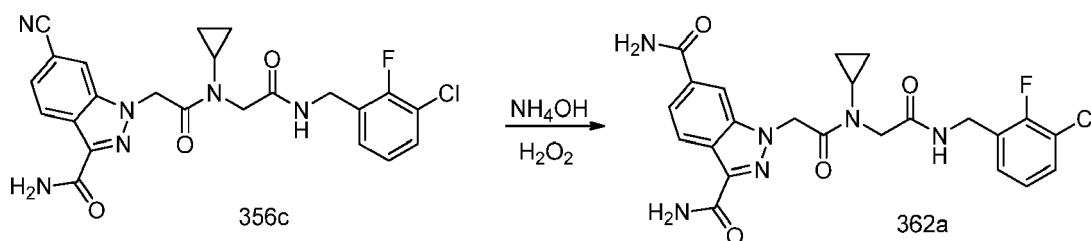
Scheme 362
