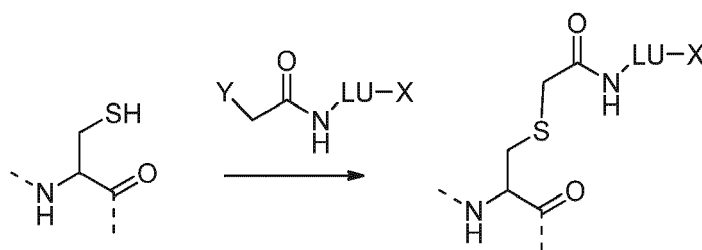
Scheme Ib. Conjugation via reaction with an alpha-halo carbonyl compound.
