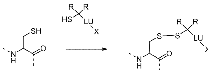
Scheme Ic. Conjugation via disulfide formation.
