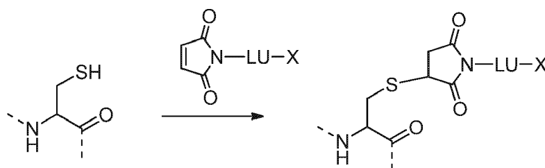
Scheme Ia. Conjugation via thiol-maleimide adduct formation.
