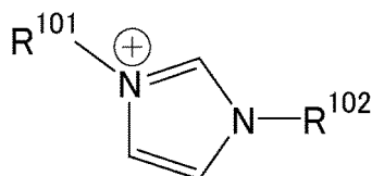
[Chem. 7]
