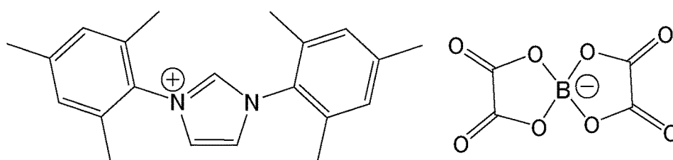
[Chem. 18]
