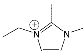
[Chem. 62]
