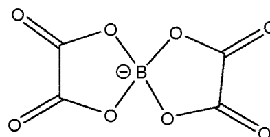
[Chem. 29]
