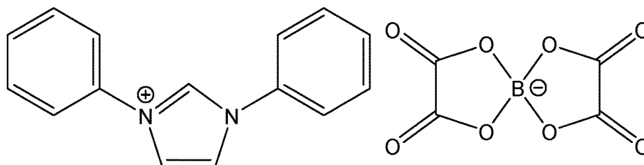
[Chem. 17]
