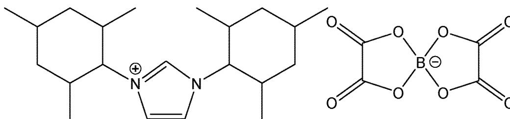
[Chem. 17]
