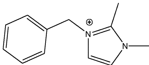
[Chem. 31]
