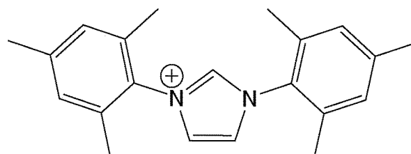
[Chem. 48]
