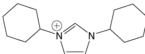
[Chem. 47]
