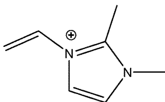
[Chem. 56]
