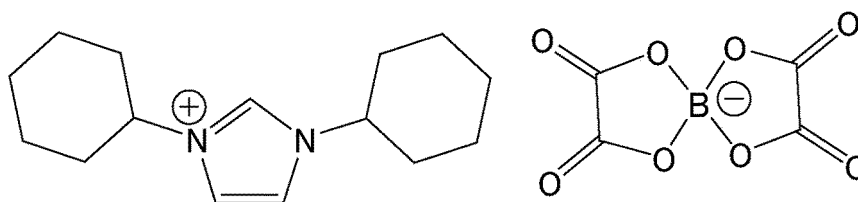
[Chem. 37]
