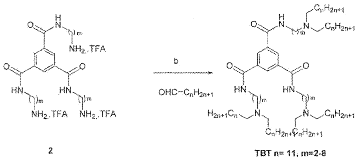
Scheme 3
