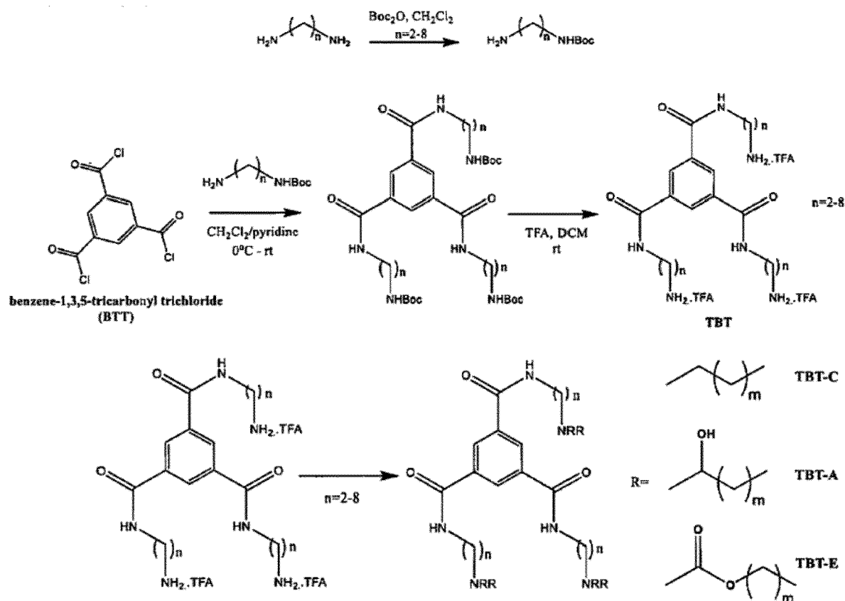
Scheme 4
