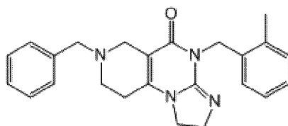
compound (1)
