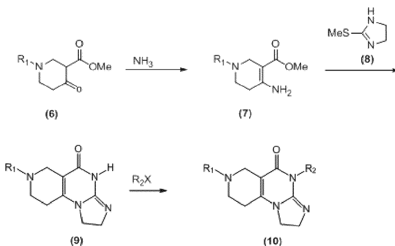
Scheme 3
