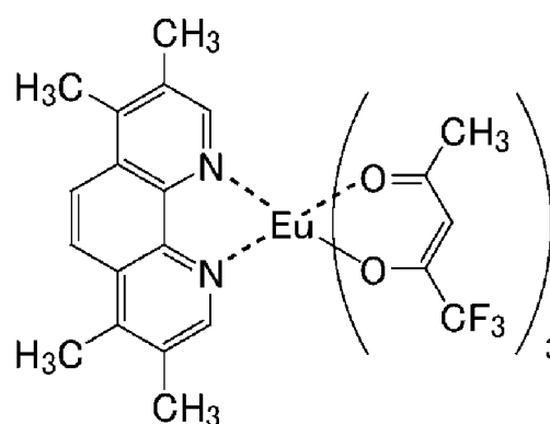
[Eu(TFA) 3 ]tmphen
