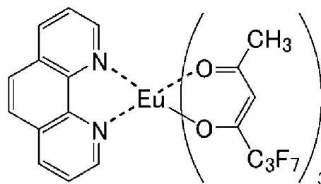
[Eu(FPD) 3 ]phen
