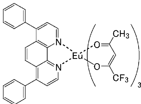
Eu(TFA) 3 dpphen
