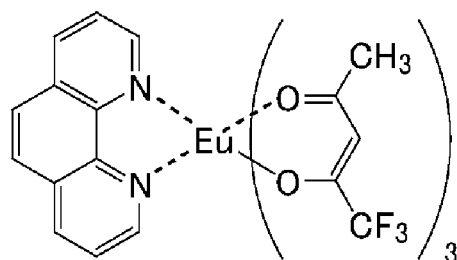
Eu(TFA) 3 phen
