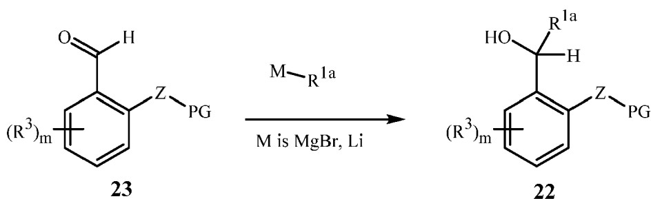
Scheme 13
