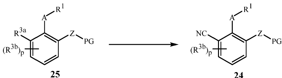
Scheme 14
