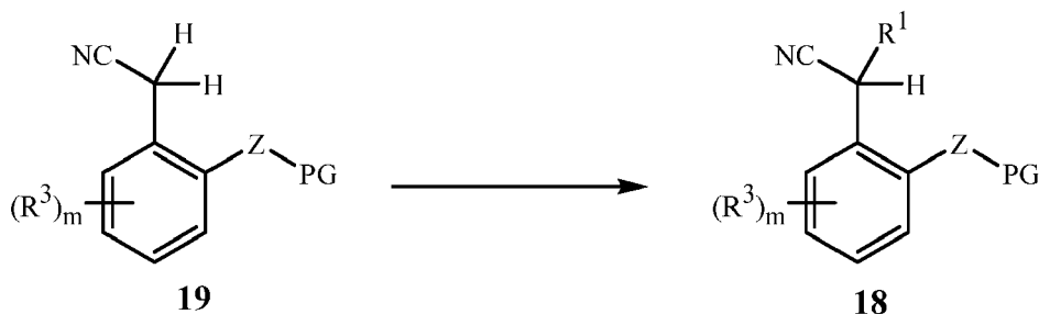
Scheme 11
