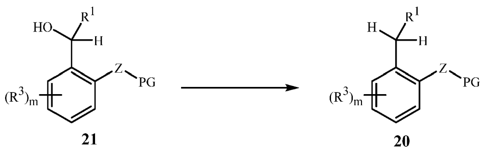
Scheme 12
