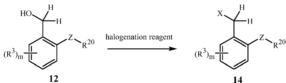
Scheme 8
