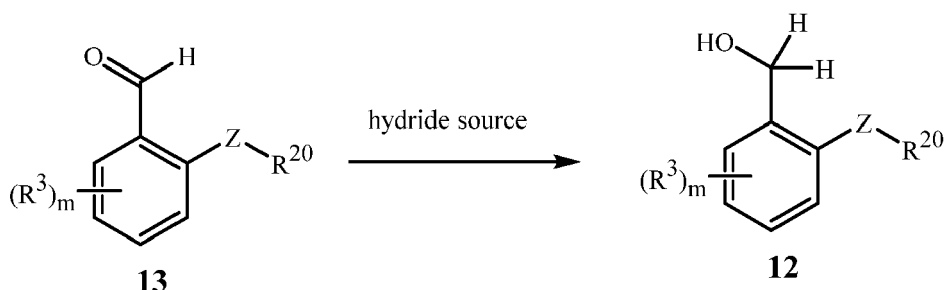
Scheme 7
