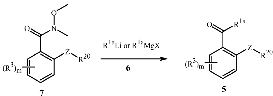
Scheme 4
