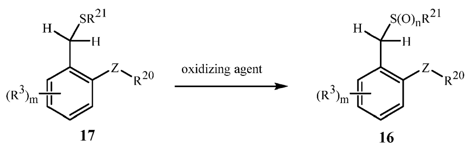
Scheme 10
