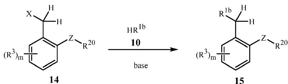
Scheme 9
