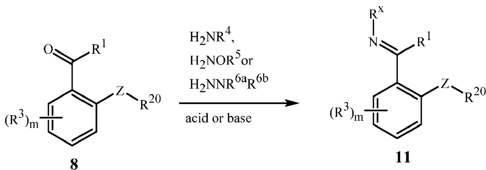
Scheme 6
