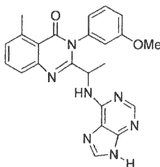
3-(3-Methoxy-phenyl)-5-methyl-2-[1-(9H-purin-6-ylamino)-ethyl]-3H-quinazolin-4-one (128)
