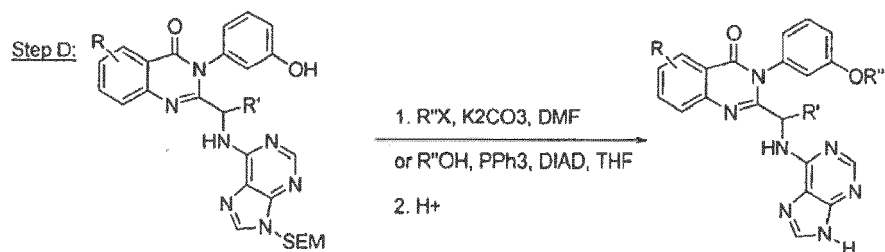
Scheme D
