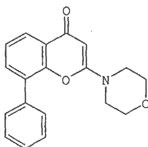
LY294002
