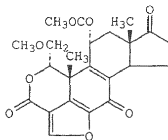
wortmannin
