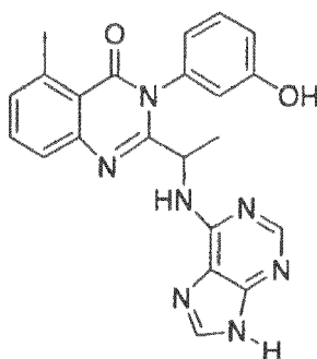
3-(3-Hydroxy-phenyl)-5-methyl-2-[1-(9H-purin-6-ylamino)-ethyl]-3H-quinazolin-4-one (121)
