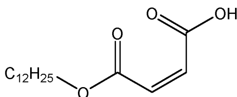
[Chemical Formula 1-1]
