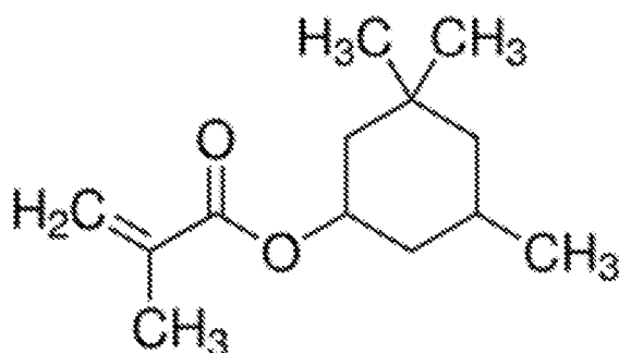
3,3,5-trimethylcyclohexyl methacrylate
