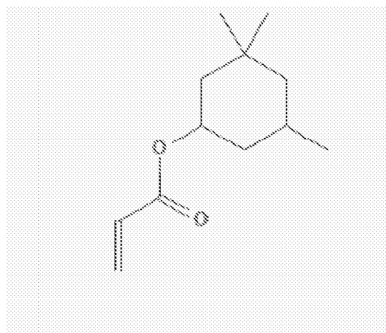
3,3,5-trimethylcyclohexyl acrylate
