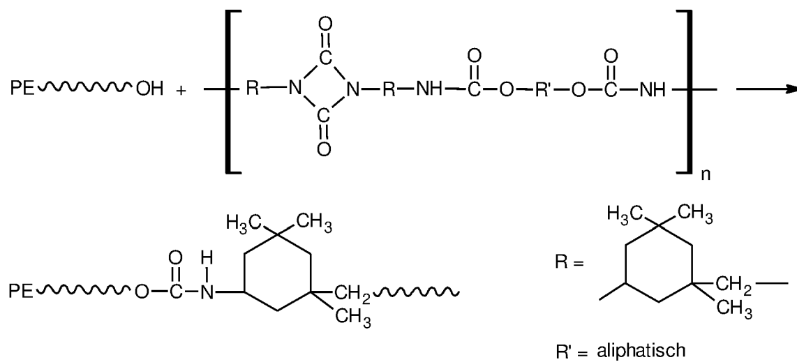
Fig. 4f Hydroxylated Polyester cured with Polyisocyanate (Polyuretdione)
