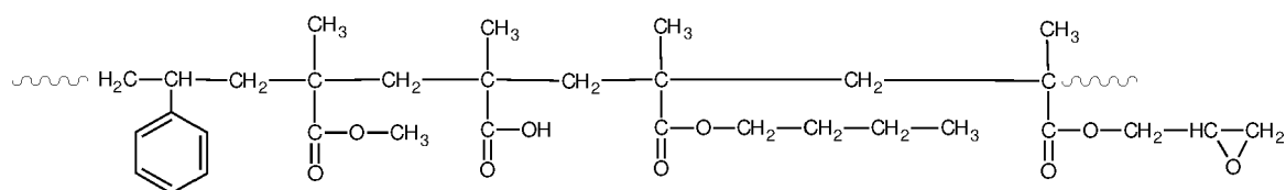
Fig.5 GMA –Acrylate resin
