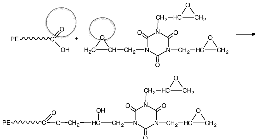
Fig.4a Carboxylated Polyester (PE) cured with TGIC
