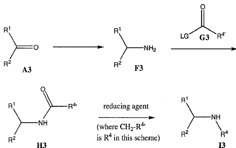
Scheme 3
