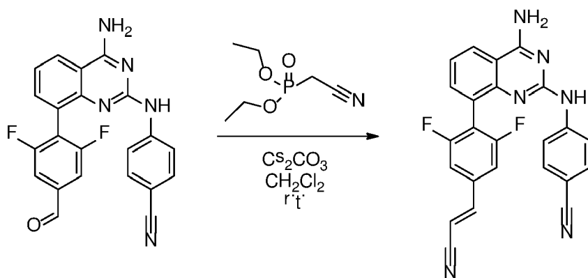
Compound 8
