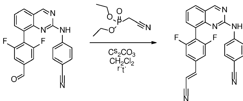
Compound 5
