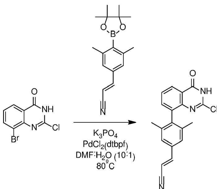
Compound 34b
