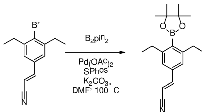
Compound 35b
