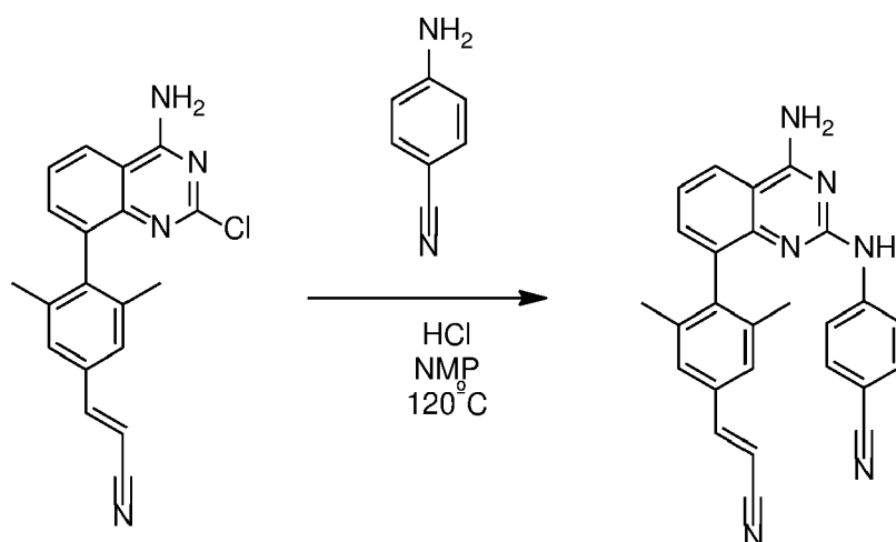
Compound 2
