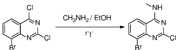
Compound 30a
