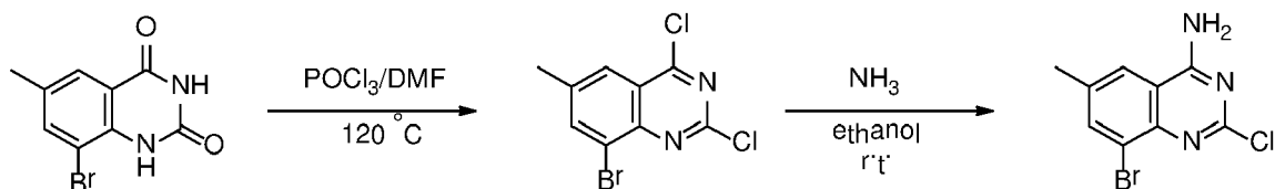
Compound 21c
