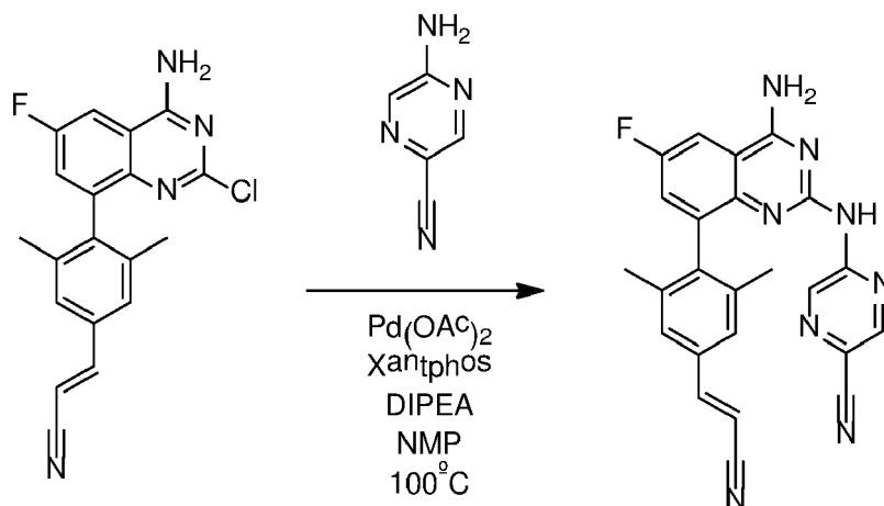
Compound 26
