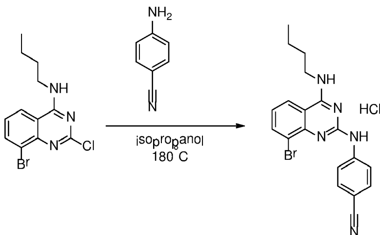
Compound 7b
