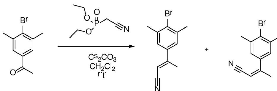
Compound 38c
