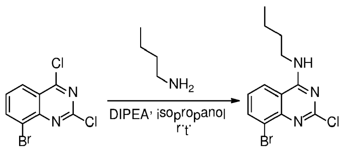
Compound 7a
