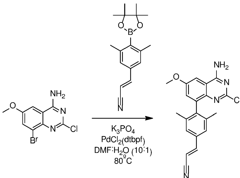
Compound 24d
