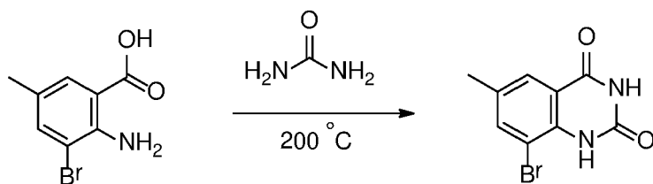
Compound 21b
