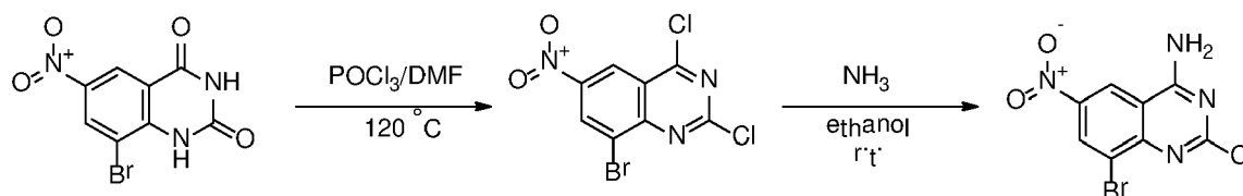
Compound 22c
