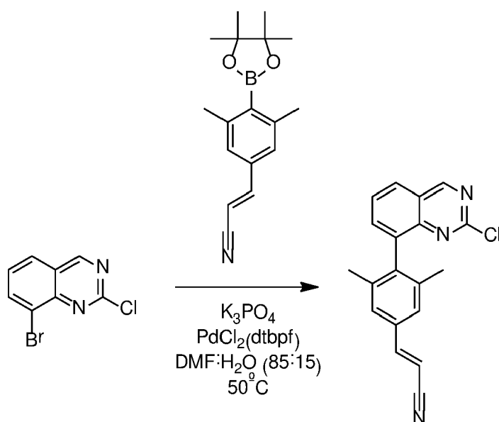
Compound 13a
