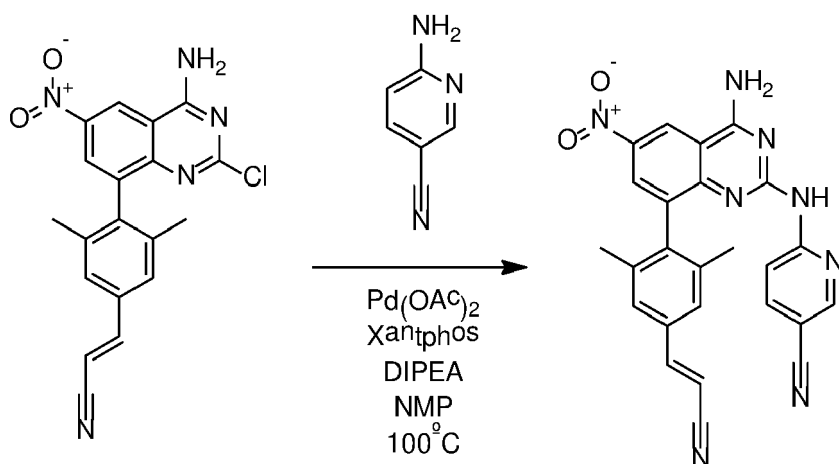
Compound 22
