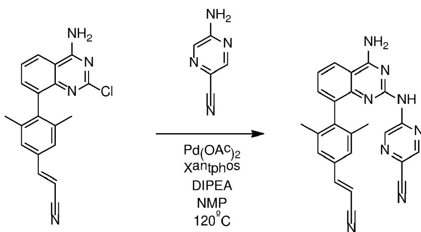
Compound 12
