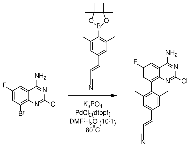
Compound 20d
