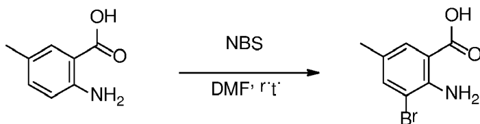
Compound 21a
