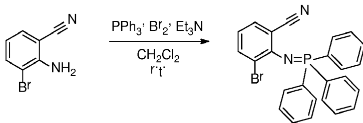
Compound 43a
