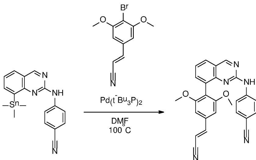
Compound 33
