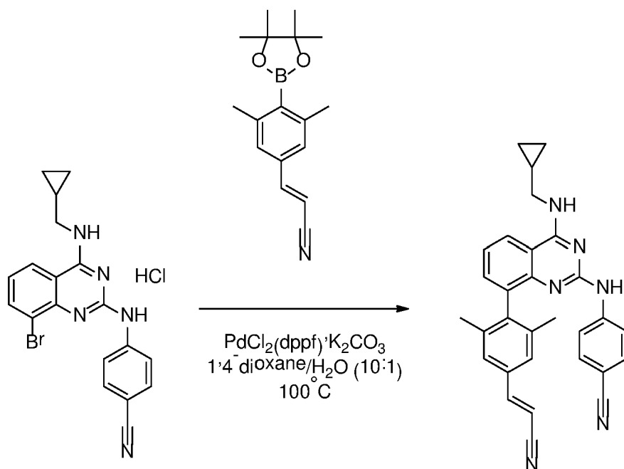
Compound 6
