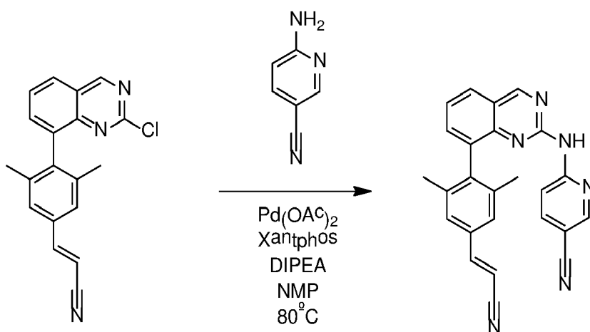
Compound 13
