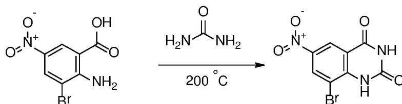
Compound 22b
