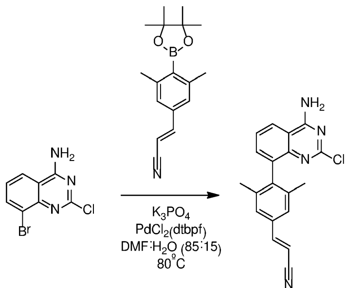
Compound 2a
