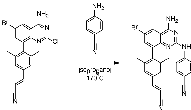
Compound 25
