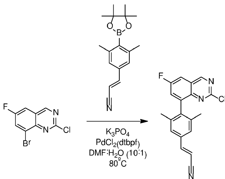
Compound 14a
