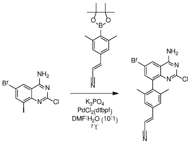
Compound 25d
