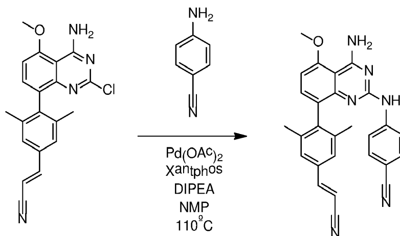
Compound 28
