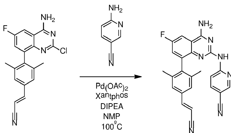
Compound 20
