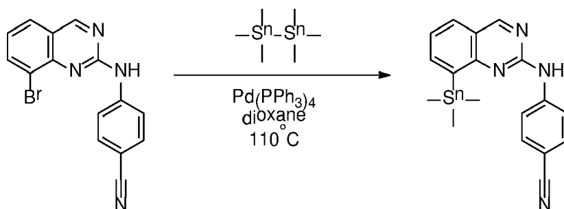
Compound 33a
