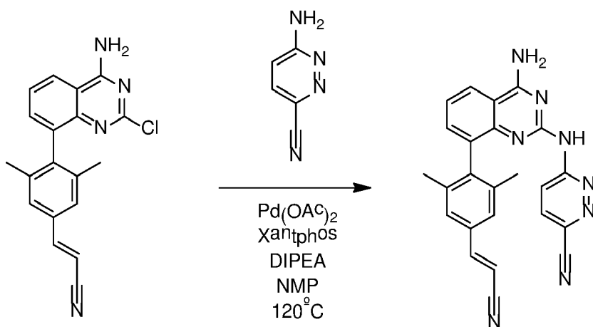
Compound 11
