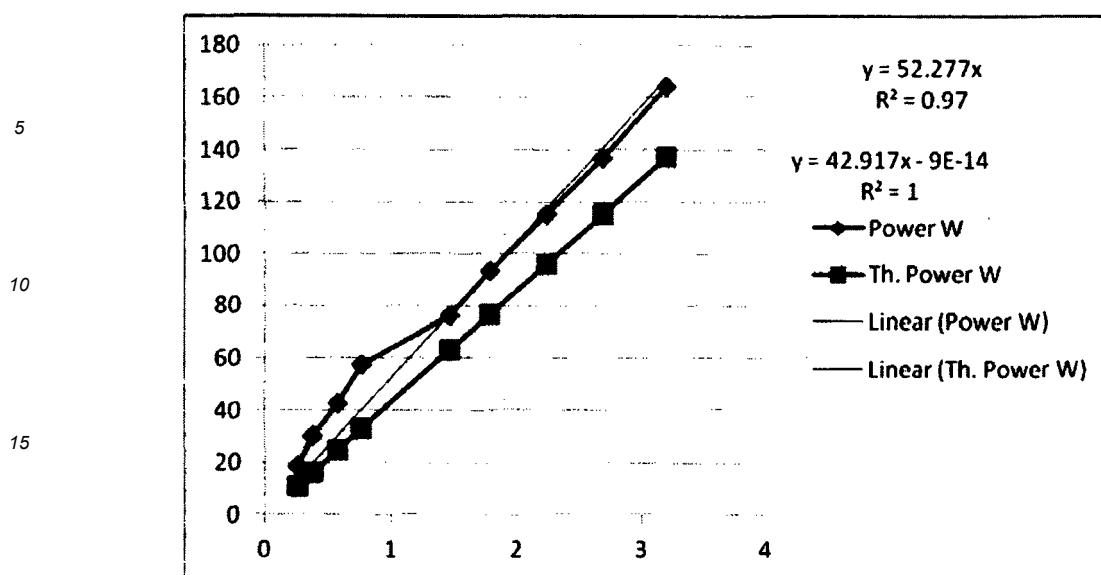
Chart 1 Empirical values of power required to vaporise the input water flow.
