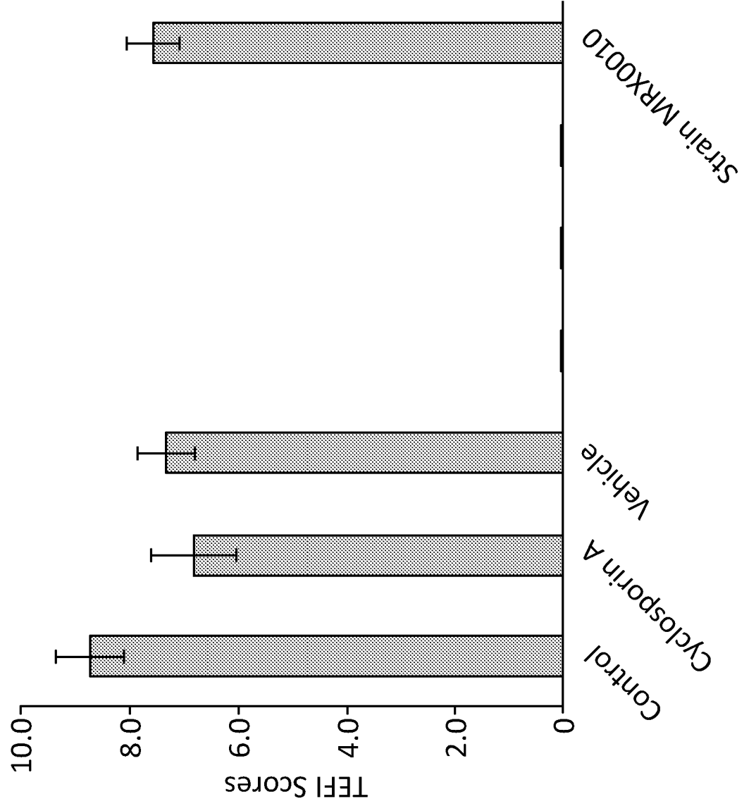
FIG. 3 TEFI Scores
