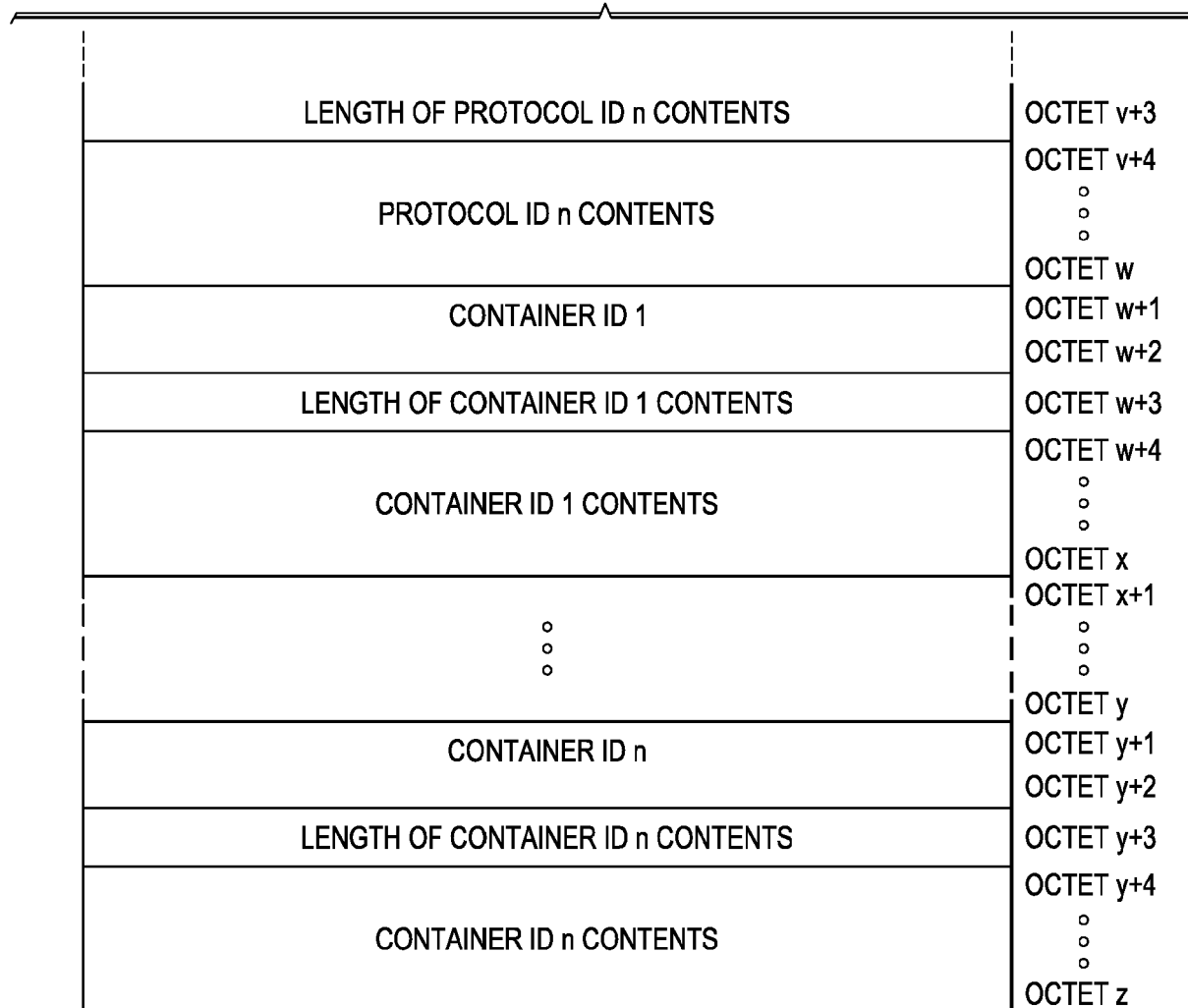
FIGURE 10.5.136/3GPP TS 24.008: PROTOCOL CONFIGURATION OPTIONS INFORMATION ELEMENT
