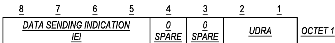
FIGURE 9.9.4.29.1: DATA SENDING INDICATION INFORMATION ELEMENT
