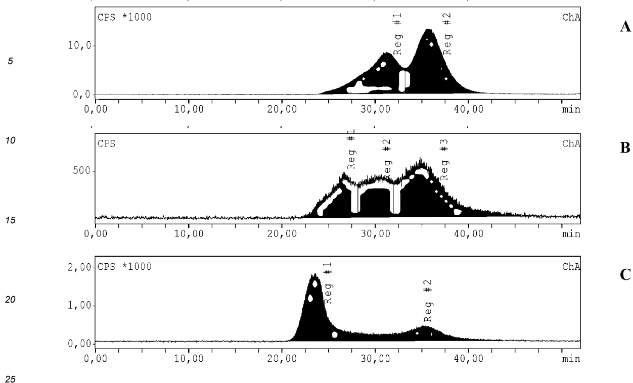
Figure 2: Size exclusion radio-chromatograms of (A) ^{177}\text{Lu} -CC49-TCO and ^{177}\text{Lu} -CC49-TCO in the presence of bovine submaxillary mucin type I-S (BSM) (B) before and (C) after 1 hr reaction with tetrazine 7
