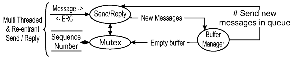
Send/Reply Data Flow Diagram
