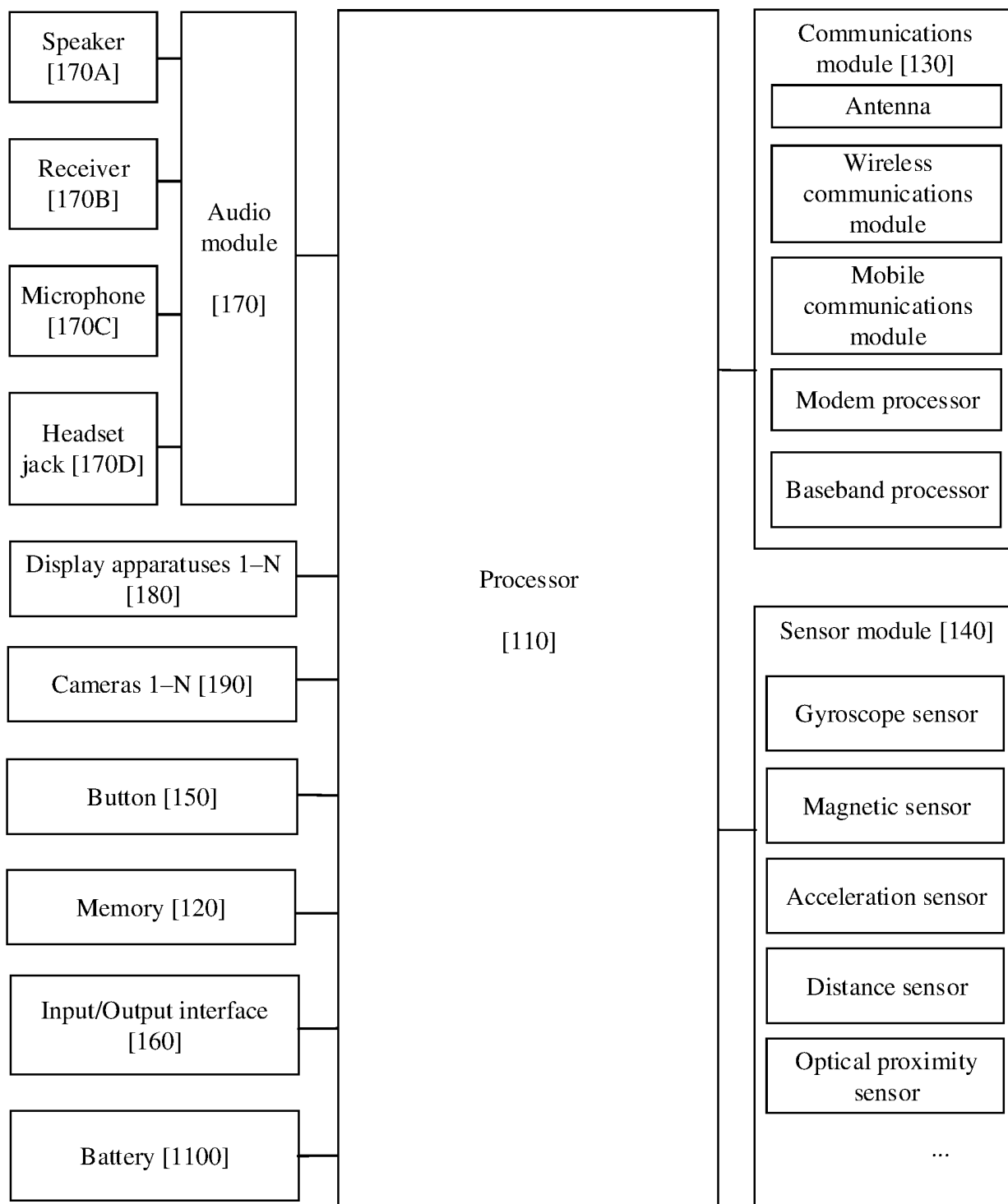
Electronic device 100
