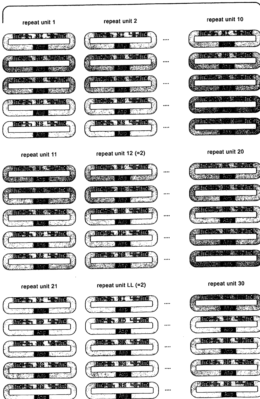
FIG. 19A insert plasmids
