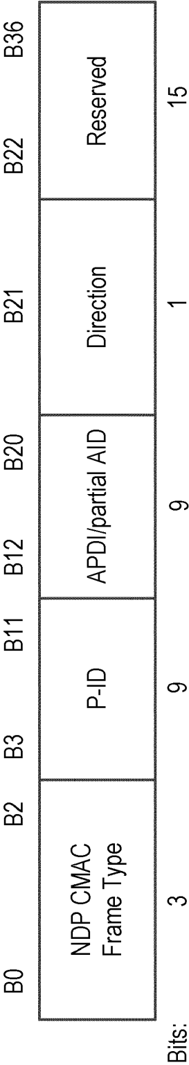
NDP CMAC frame body field of the NDP_2M Paging frame
