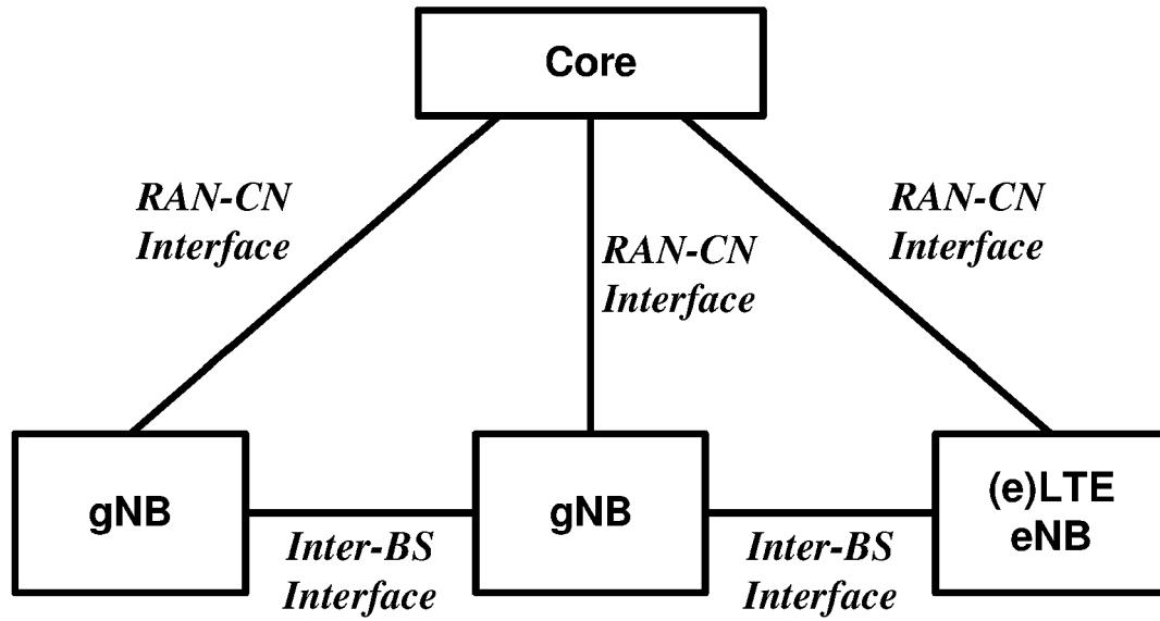
Non-centralized deployment
