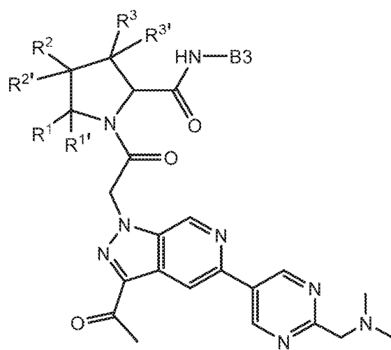
Formula I-176
