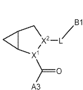
Formula I-10
