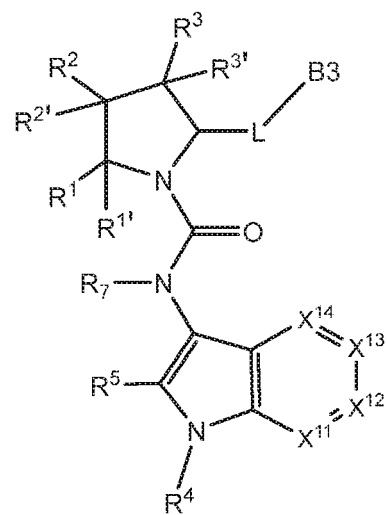
Formula I-15
