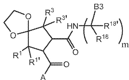
Formula I-23
