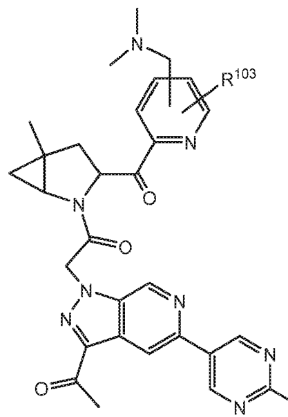
Formula I-105
