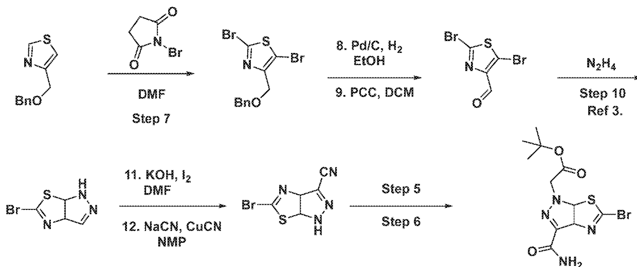
Scheme 6 continued
