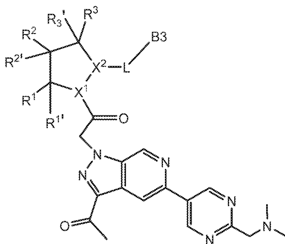
Formula I-174
