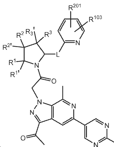
Formula I-138
