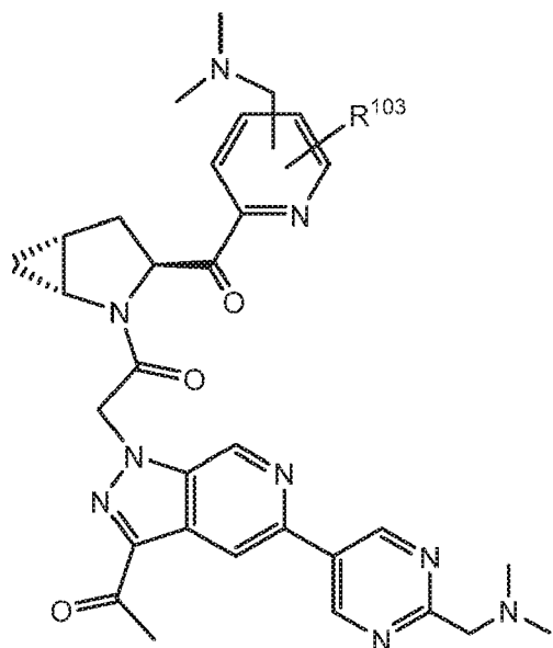
Formula I-206
