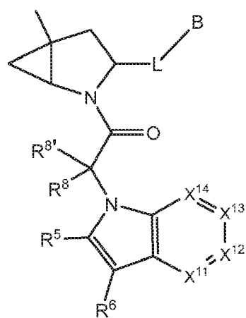
Formula II-16
