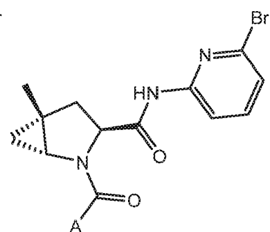
Formula I-58
