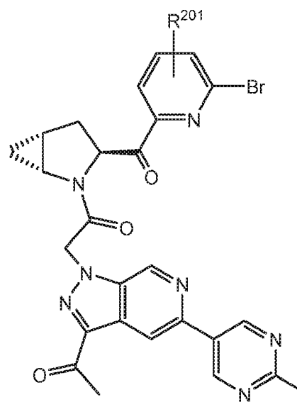
Formula I-101
