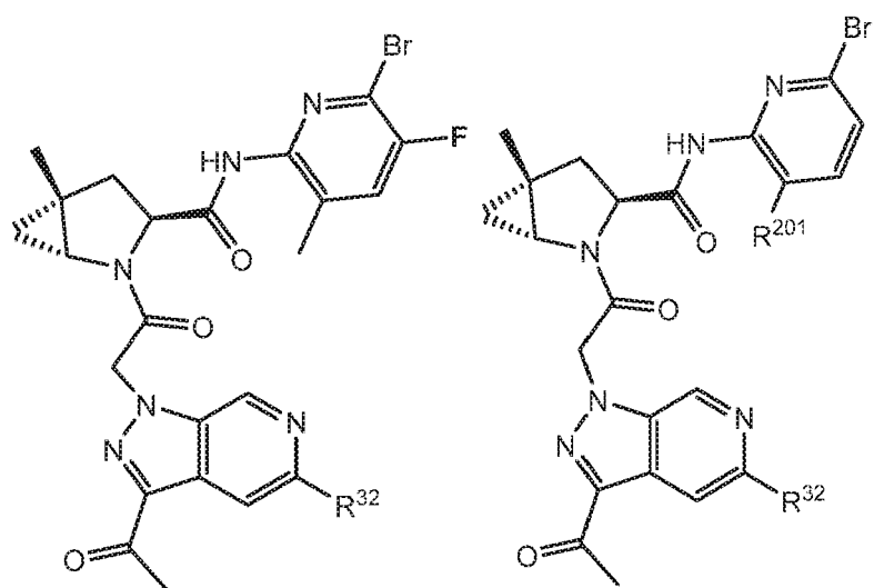
Formula I-229
