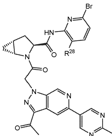
Formula I-110
