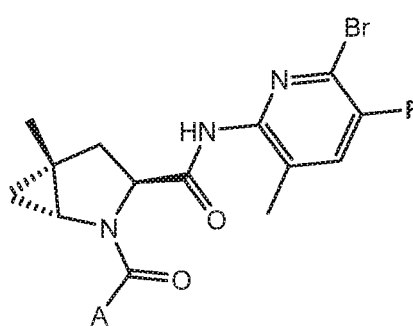
Formula I-60
