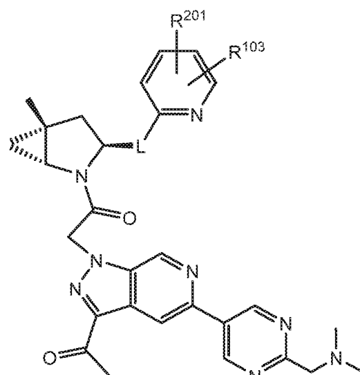
Formula II-120
