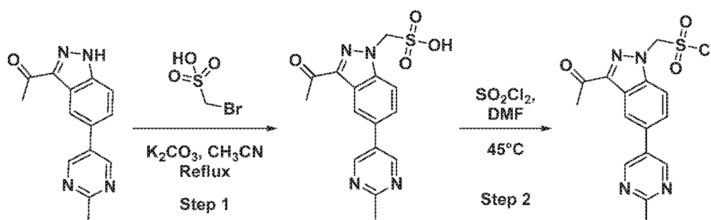
Scheme 7-1
