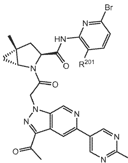
Formula I-116
