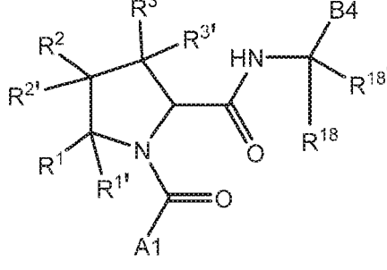
Formula III-5
