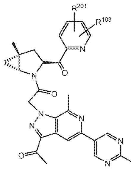
Formula II-94
