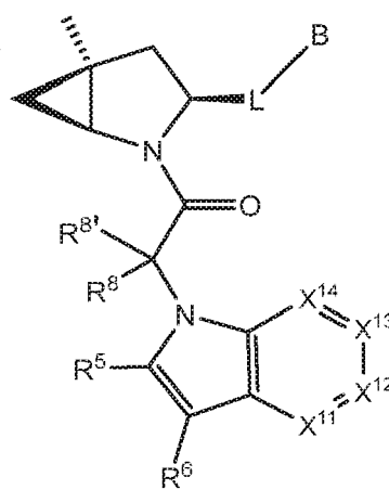
Formula I-73
