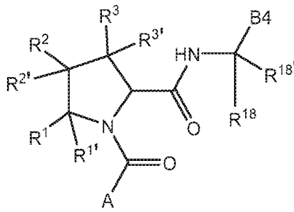
Formula III-2
