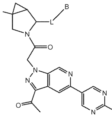
Formula II-54
