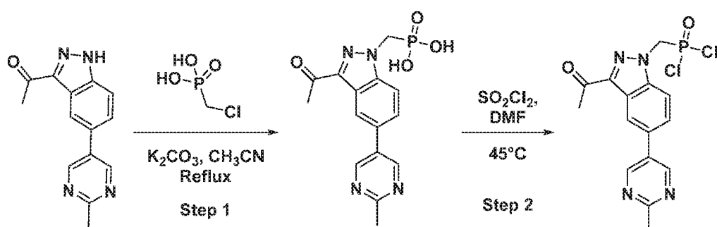
Scheme 7-2
