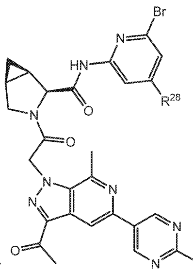
Formula I-170
