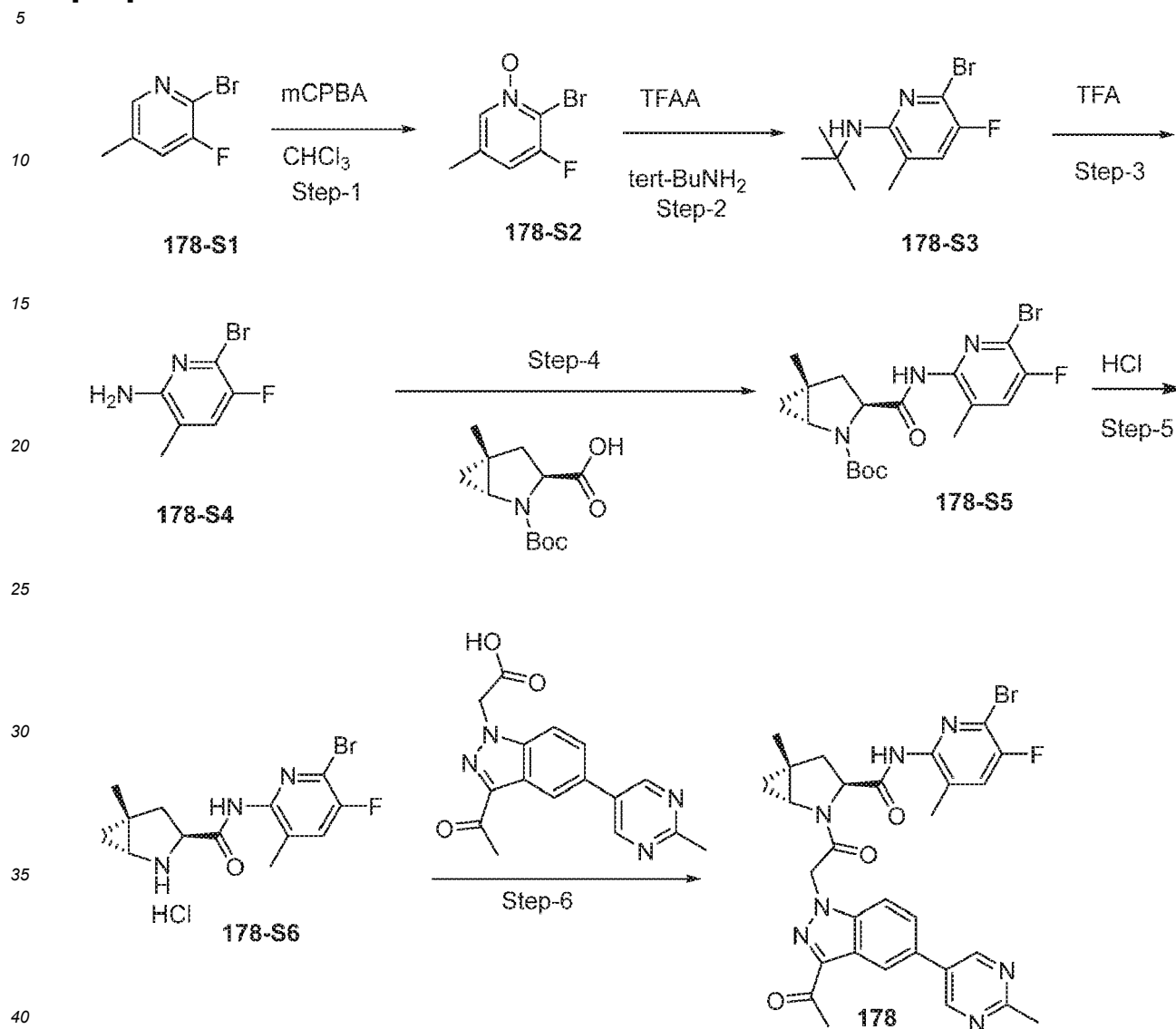
Scheme 71. Synthesis of (1 R ,3 S ,5 R )-2-(2-(3-Acetyl-5-(2-methylpyrimidin-5-yl)-1 H -indazol-1-yl)acetyl)- N -(6-bromo-5-fluoro-3-methylpyridin-2-yl)-5-methyl-2-azabicyclo[3.1.0]hexane-3-carboxamide (178)
