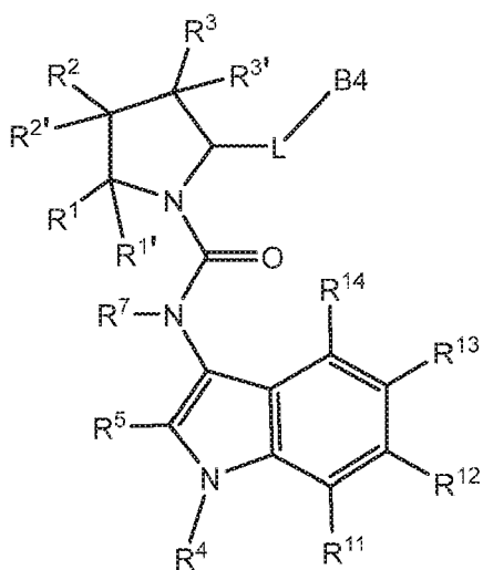
Formula III-16
