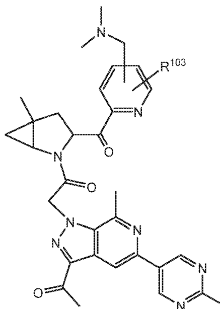
Formula II-101
