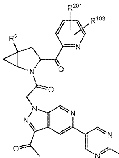
Formula I-91
