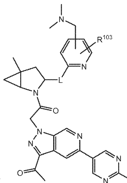
Formula II-72
