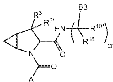
Formula I-21
