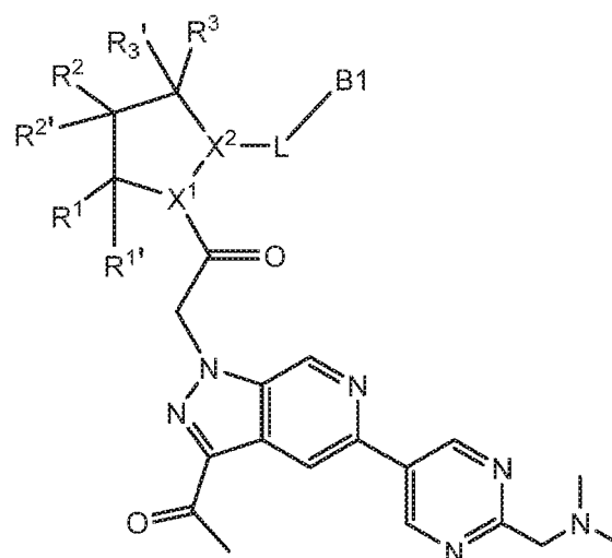
Formula I-177
