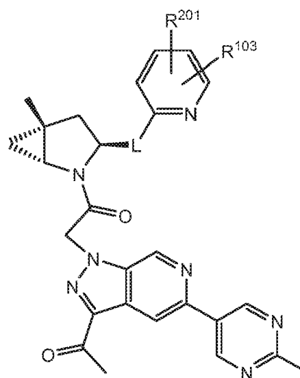
Formula II-66
