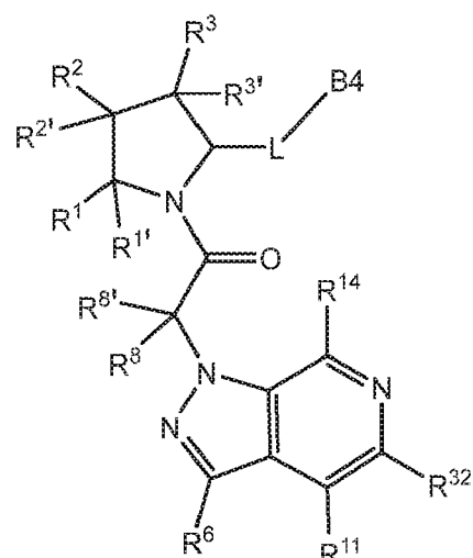
Formula III-19
