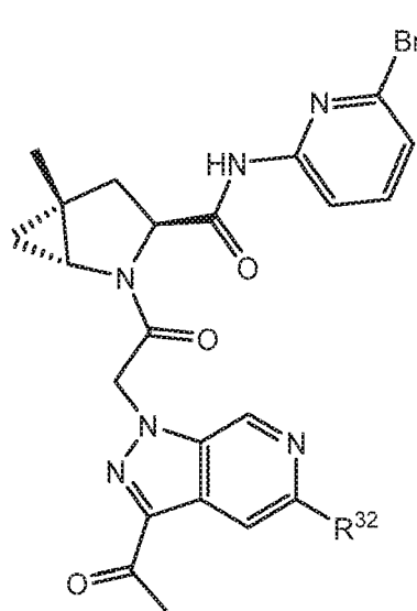
Formula I-227
