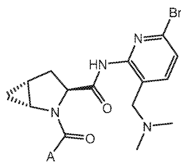
Formula I-57
