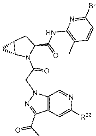
Formula I-224
