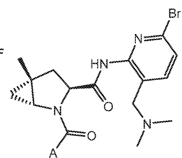
Formula I-61
