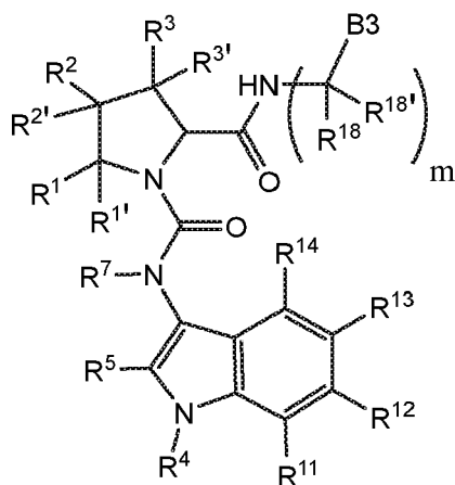
Formula I-26
