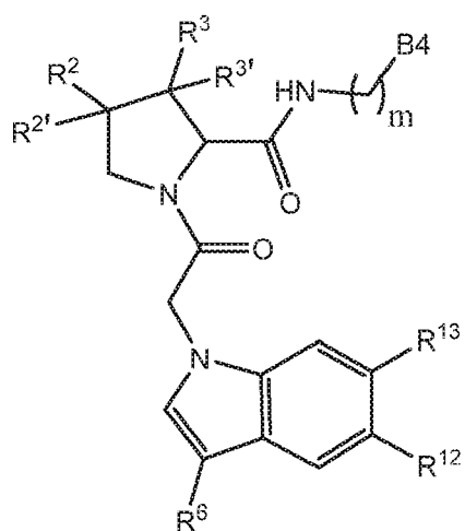
Formula III-30
