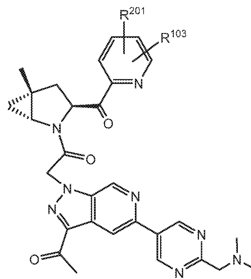
Formula I-191
