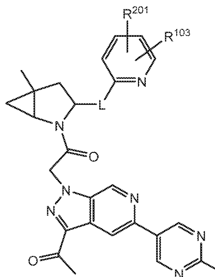
Formula II-64
