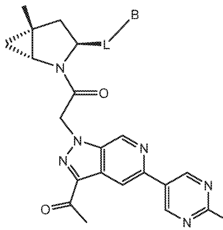
Formula II-52
