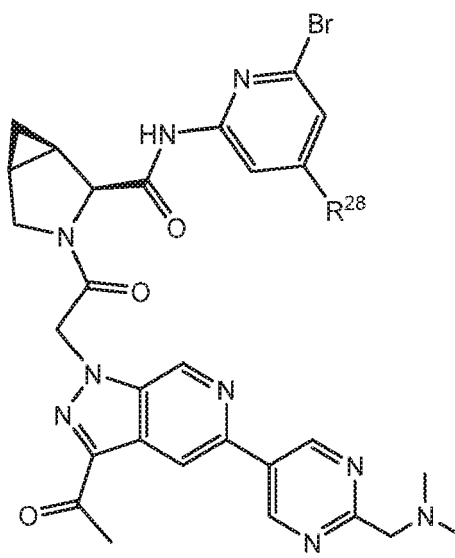
Formula I-219
