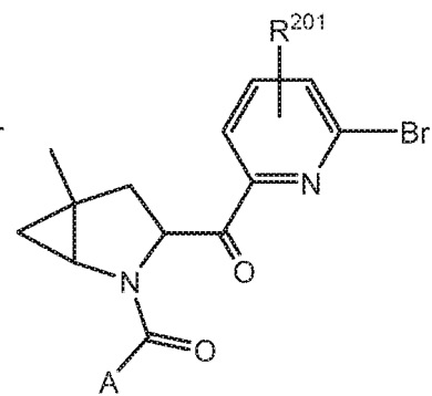
Formula I-43
