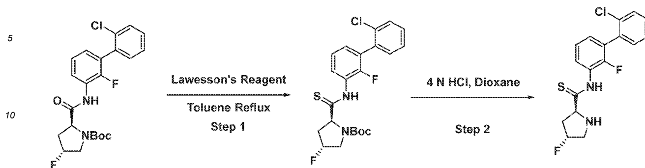
Scheme 5-4
