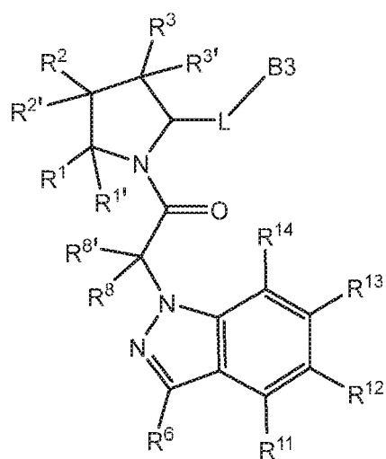
Formula I-18
