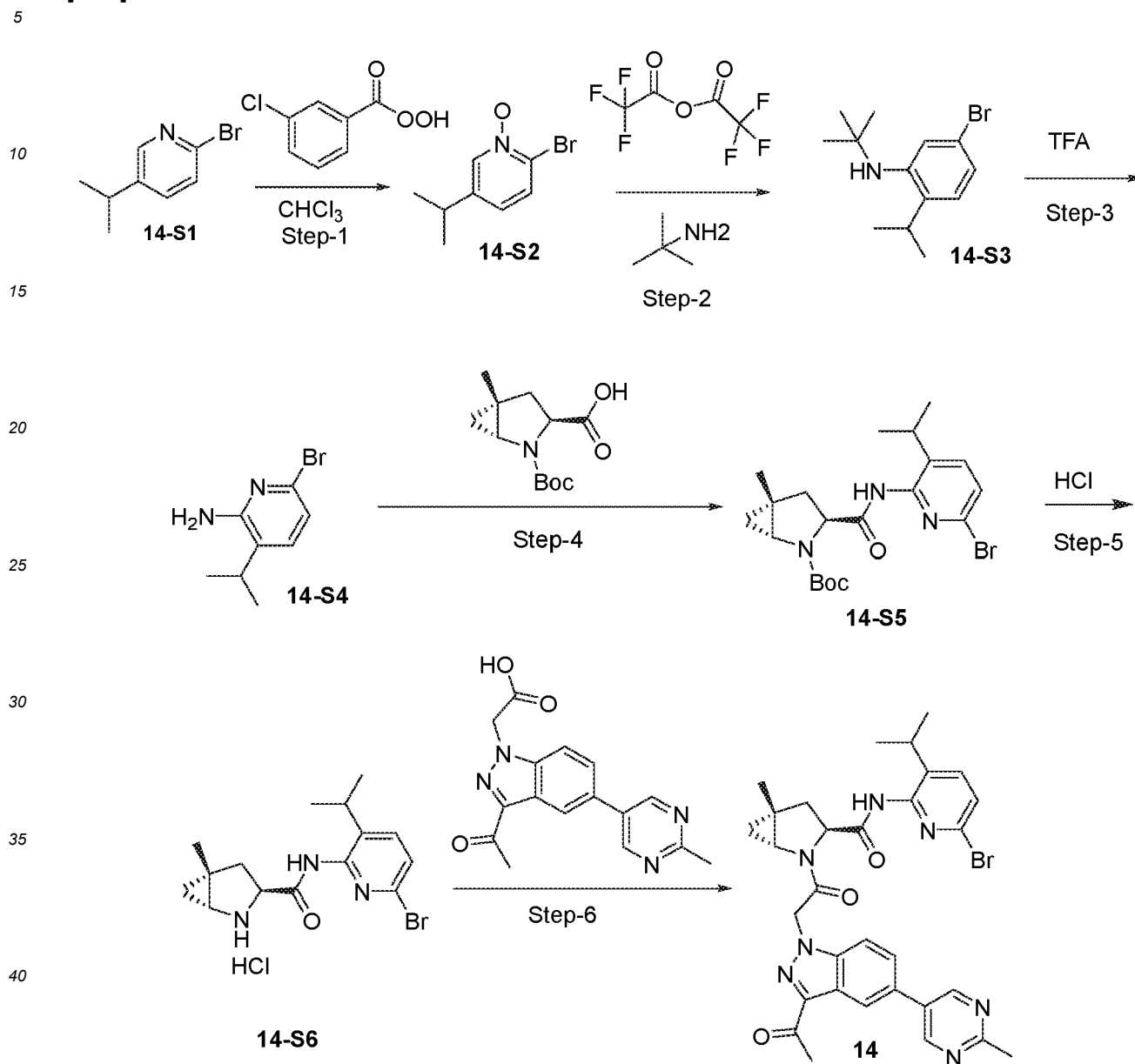
Scheme 9. Synthesis of (1 R ,3 S ,5 R )-2-(2-(3-Acetyl-5-(2-methylpyrimidin-5-yl)-1 H -indazol-1-yl)acetyl)- N -(6-bromo-3-isopropylpyridin-2-yl)-5-methyl-2-azabicyclo[3.1.0]hexane-3-carboxamide (14)
