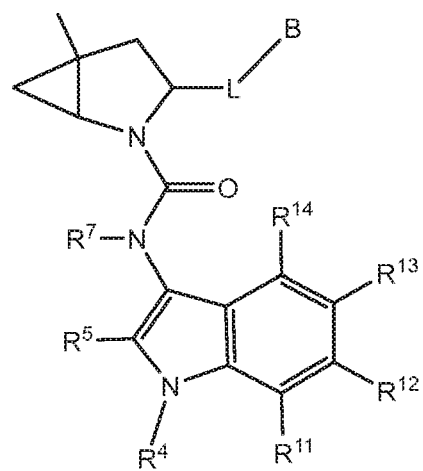
Formula II-16
