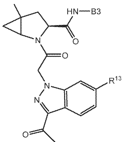
Formula II-35
