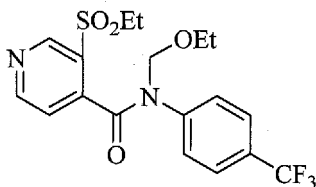
Compound B
