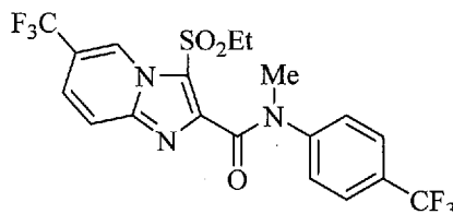
Compound A
