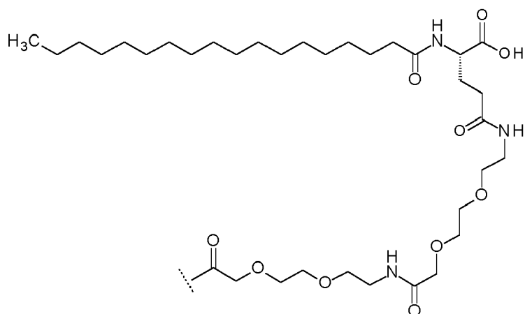
(iv) Eicosanoyl-isoGlu-Peg3-Peg3
