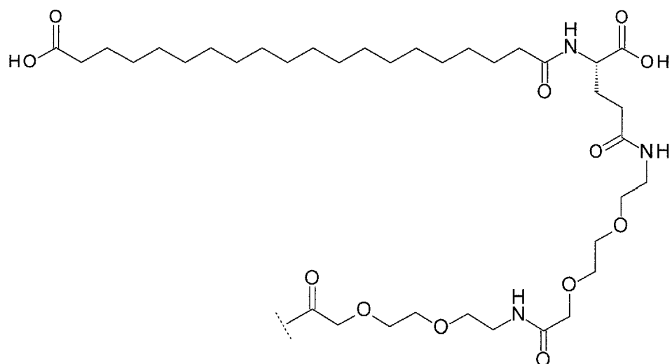
(vi) Octadecanoyl-Dapa-Peg3-Peg3
