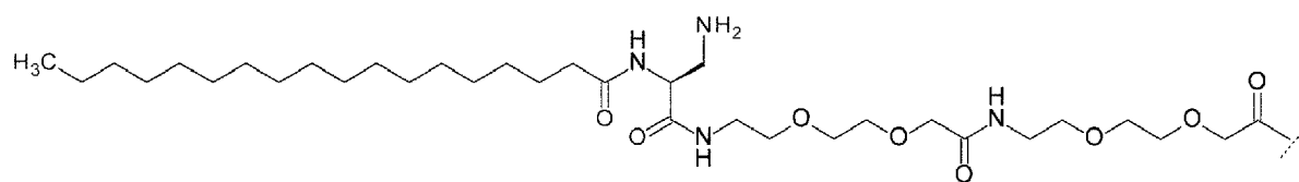
(vii) Hexadecanoyl-isoGlu
