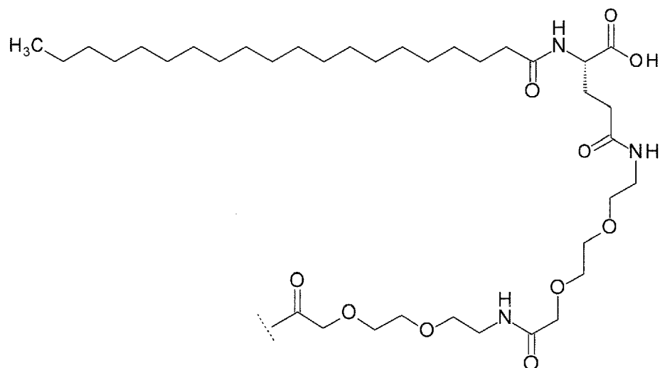
(v) [19-carboxy-nonadecanoyl]-isoGlu-Peg3-Peg3
