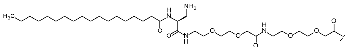
(vii) Hexadecanoyl-isoGlu
