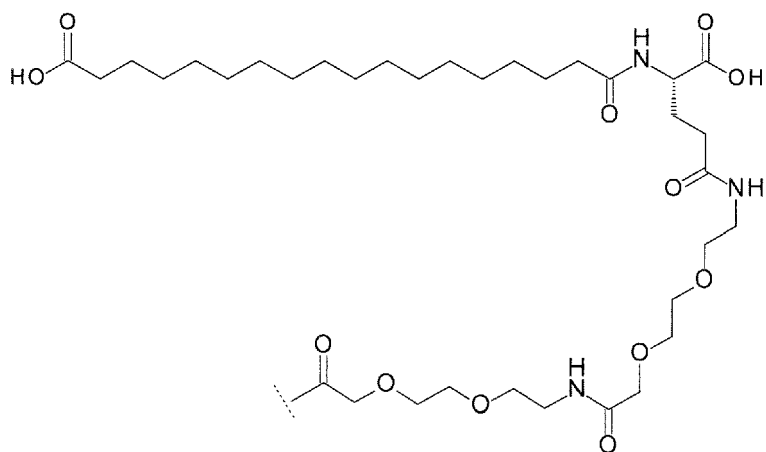
(ii) [17-carboxy-heptadecanoyl]-isoGlu
