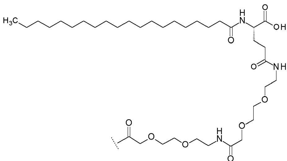
(v) [19-carboxy-nonadecanoyl]-isoGlu-Peg3-Peg3
