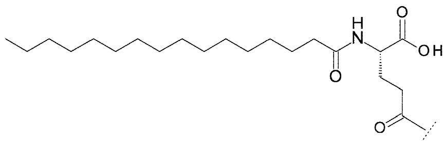
(vii) Hexadecanoyl-isoGlu
