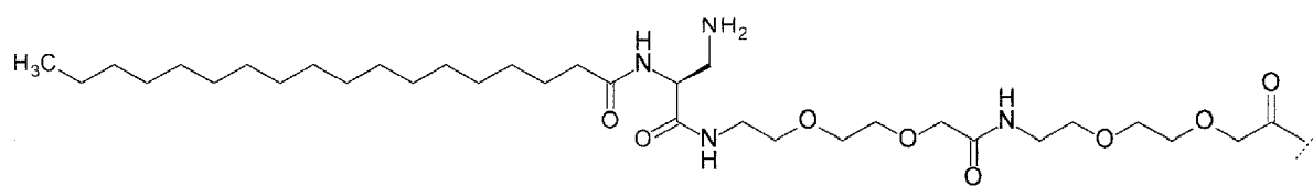
(vii) Hexadecanoyl-isoGlu
