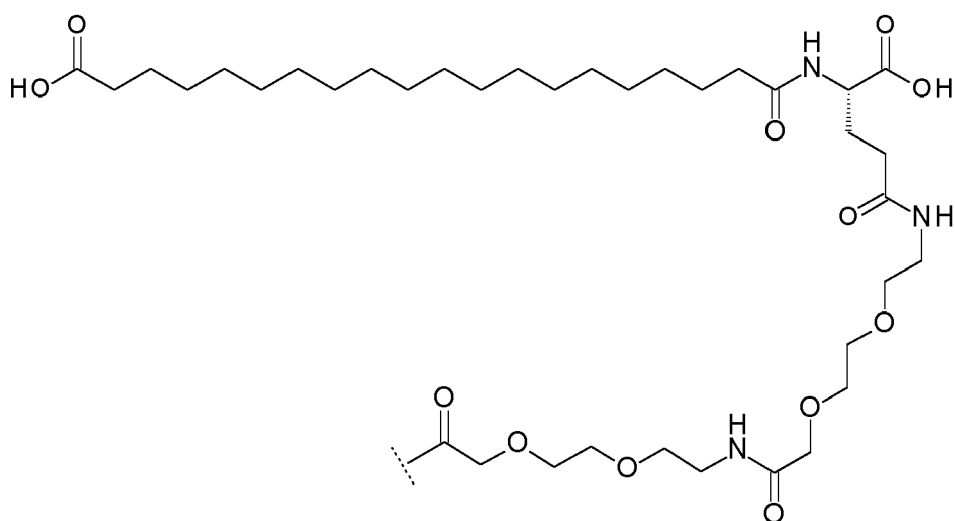
(vi) Octadecanoyl-Dapa-Peg3-Peg3
