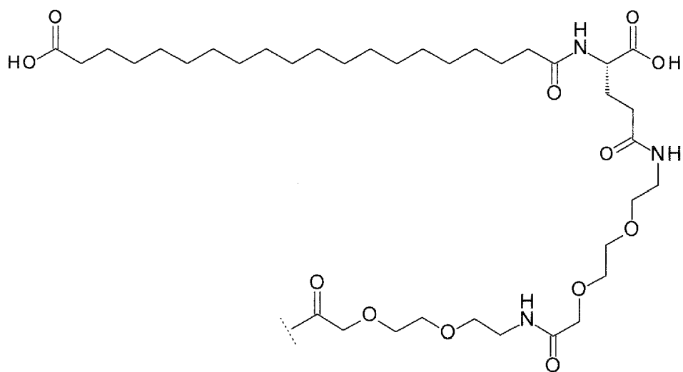
(vi) Octadecanoyl-Dapa-Peg3-Peg3
