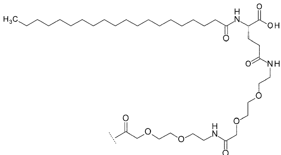
(v) [19-carboxy-nonadecanoyl]-isoGlu-Peg3-Peg3
