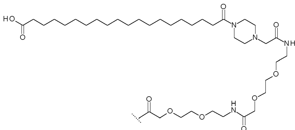
(viii) (19-Carboxy-nonadecanoyl)-[(Piperazine-1-yl)-acetyl]-Peg3-Peg3
