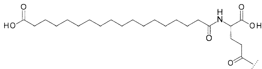
(iii) Octadecanoyl-isoGlu-Peg3-Peg3
