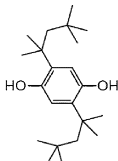
Hydroquinone compound 7 [2,5-Bis(1,1,3,3-tetramethylbutyl)hydroquinone]
