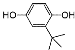
Hydroquinone compound 1 [tert-Butylhydroquinone]
