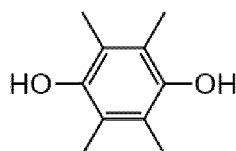
Hydroquinone compound 8 [Tetramethylhydroquinone]
