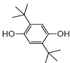
Hydroquinone compound 4 [2,5-Di-tert-butylhydroquinone]
