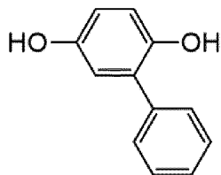
Hydroquinone compound 2 [Phenylhydroquinone]
