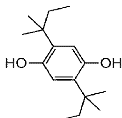
Hydroquinone compound 5 [2,5-Di-tert-amylhydroquinone]
