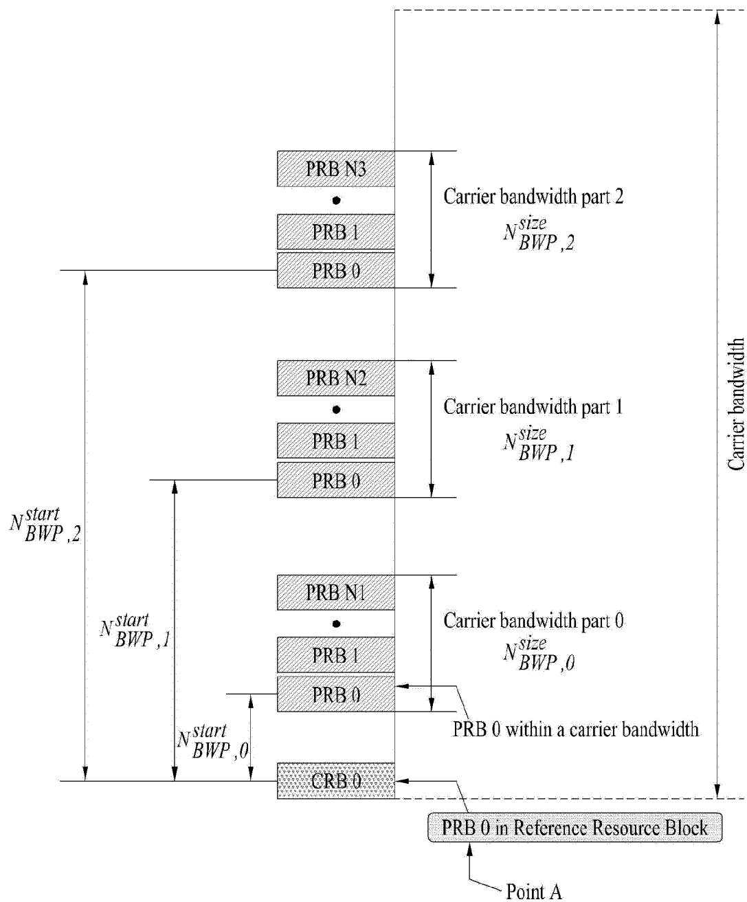
An Example of carrier bandwidth and BWP for NR
