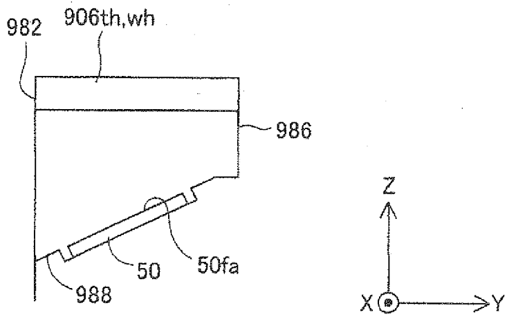
45-45 CROSS-SECTIONAL VIEW
