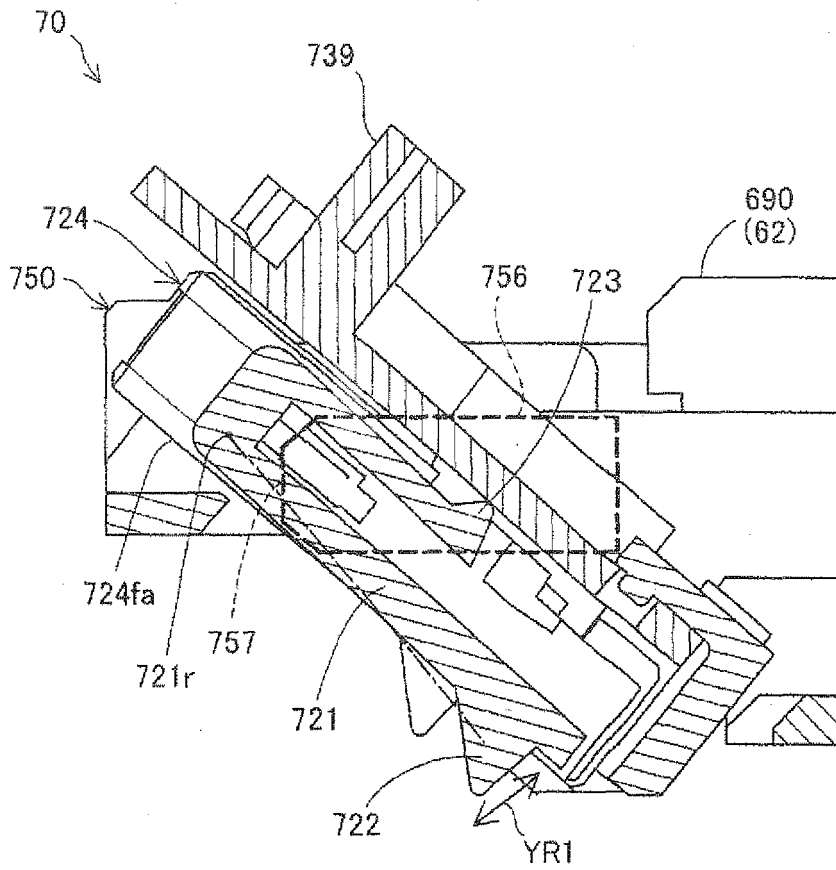
17-17 CROSS-SECTIONAL VIEW
