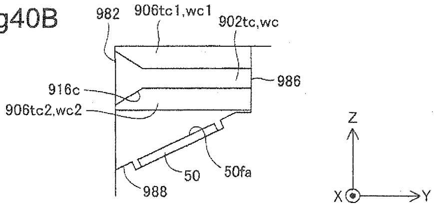
40-40 CROSS-SECTIONAL VIEW
