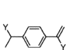
[Chem. 18]
