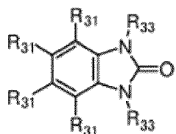
[Chem. 19]
