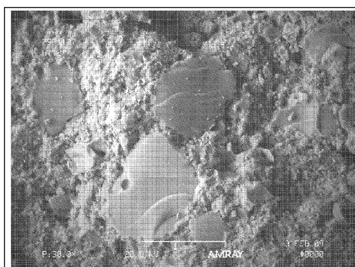
Figure 2: Scanning electron micrograph of a grout-aerogel composite.
