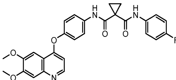
Compound I
