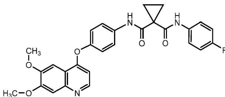
Compound I
