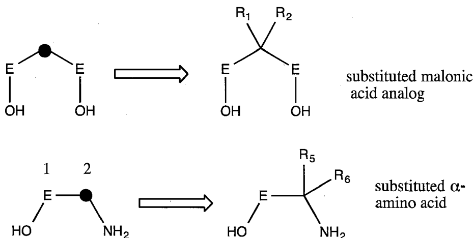
Schematic 1: Replacement of a single variable position by a -C(R_a)(R_b)- unit.
